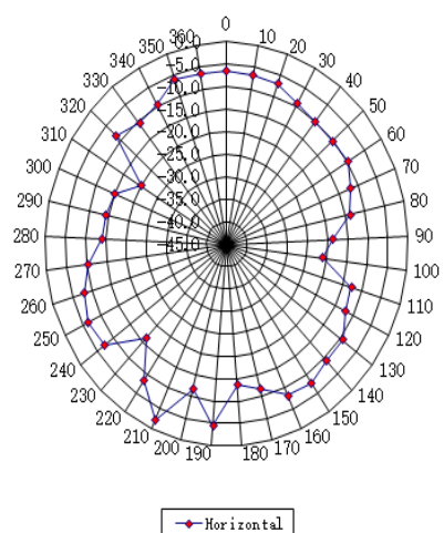
Horizontal at 2480MHz
