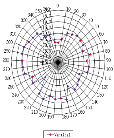
Vertical at 2480MHz
