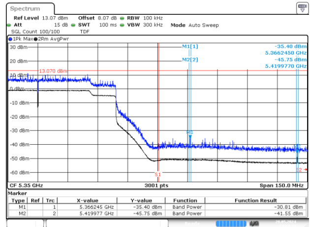
BE-R-HIGH, SISO-A, 802.11ax/be80-MCS0, Ch58
