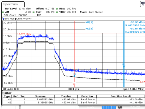
BE-R-HIGH, SISO-A, 802.11ax/be40-MCS0, Ch62
