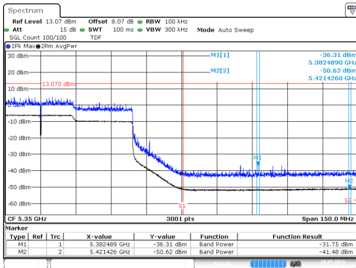
BE-R-HIGH, SISO-A, 802.11ax/be160-MCS0, Ch50
