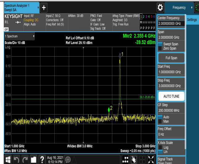
Band7-15MHz-16QAM-20825-75RB#0-Range2:1000~3000MHz
