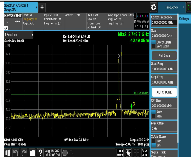
Band7-15MHz-QPSK-21375-75RB#0-Range2:1000~3000MHz
