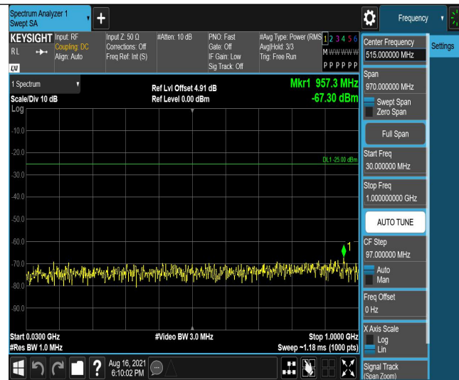
Band7-15MHz-16QAM-20825-75RB#0-Range1:30~1000MHz
