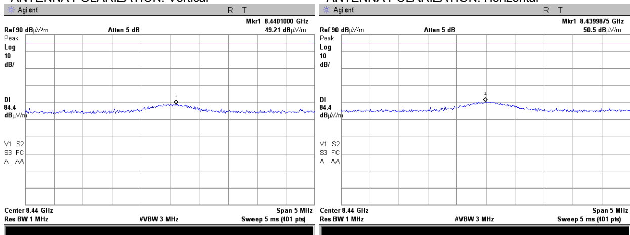
Plot 7.7.14 Radiated emission measurements at the 4 th harmonic
