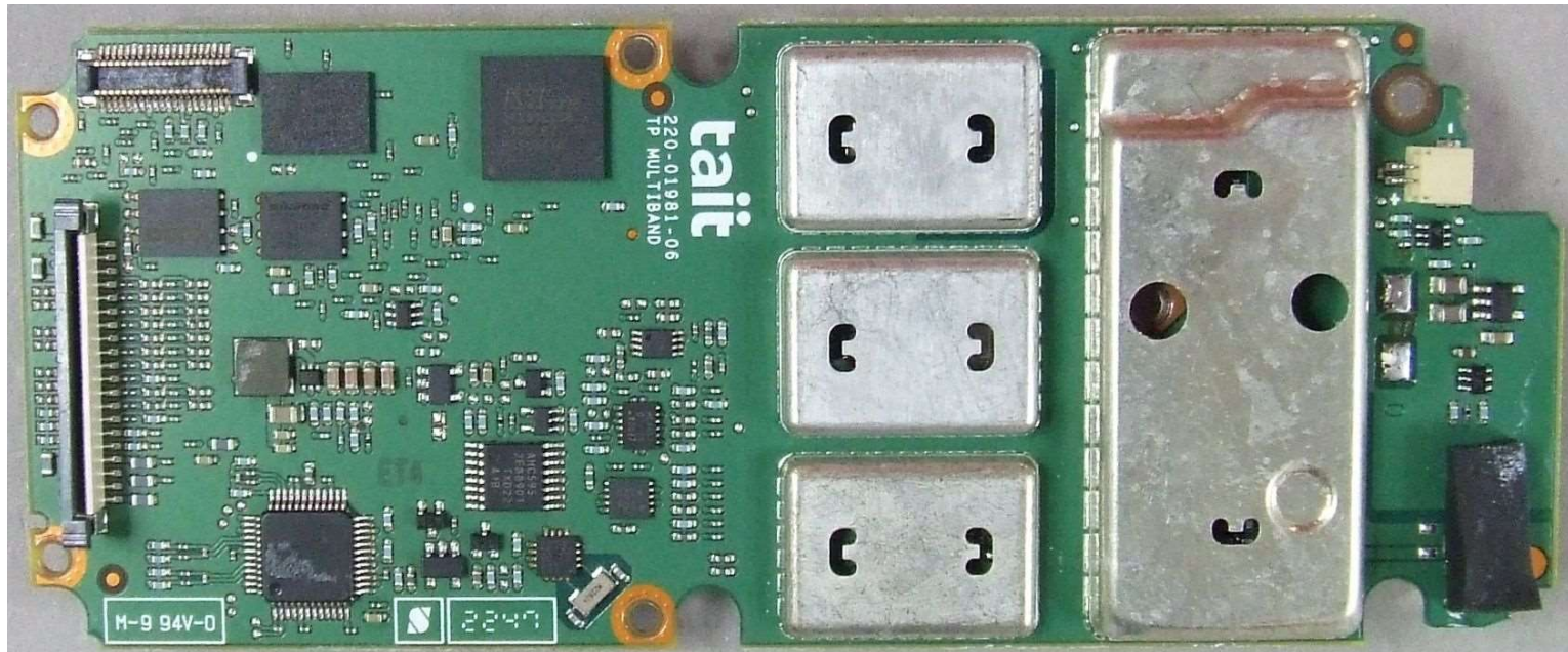
Photograph 01: Receive-Transmit PCB – top (with shields)
