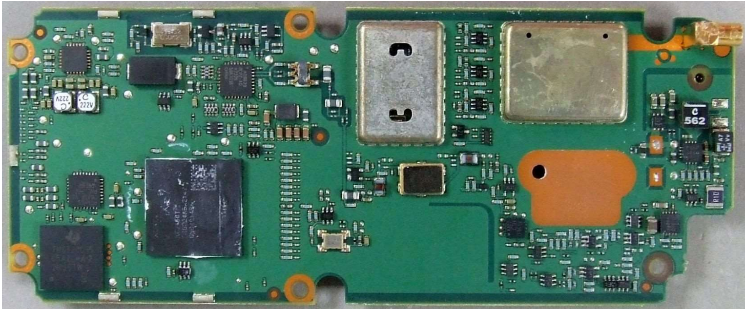
Photograph 03: Receive-Transmit PCB - bottom (with shields)
