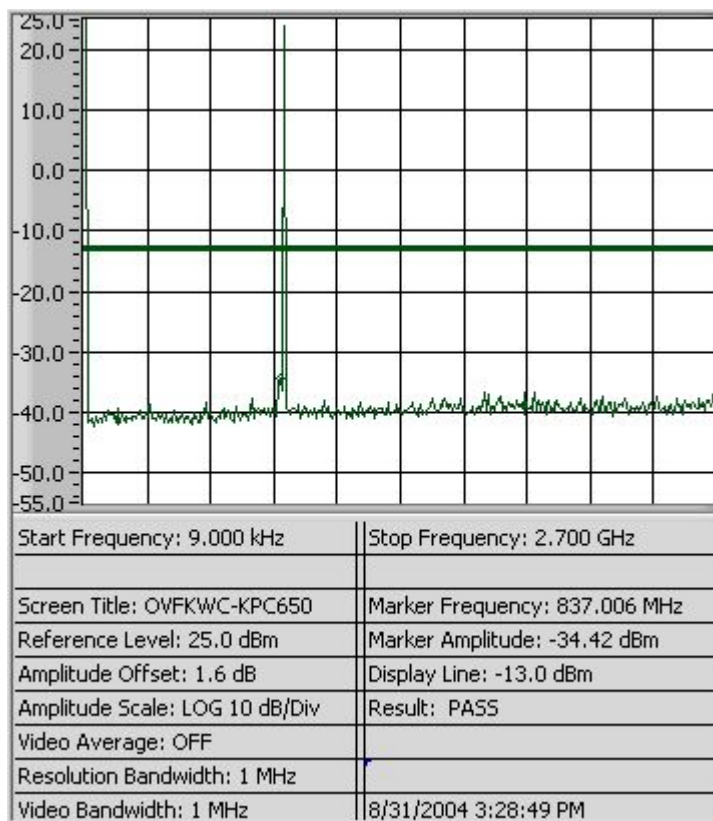
Figure 8-2a CDMA 800 – Conducted Spurious Emission (CH 1013)
