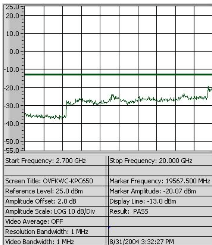
Figure 8-9b CDMA 1900 - Conducted Spurious Emission (CH 1175)
