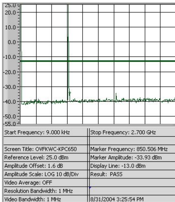
Figure 8-6a CDMA 800 – Conducted Spurious Emission (CH 777)
