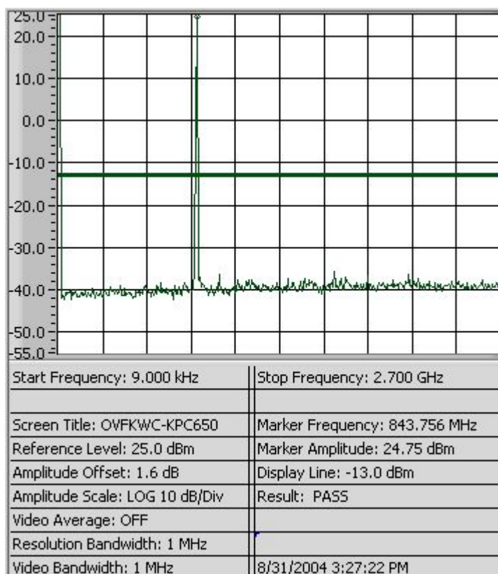
Figure 8-4a CDMA 800 – Conducted Spurious Emission (CH 383)
