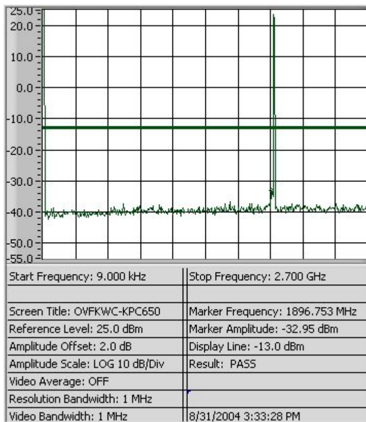
Figure 8-8a CDMA 1900 - Conducted Spurious Emission (CH 600)
