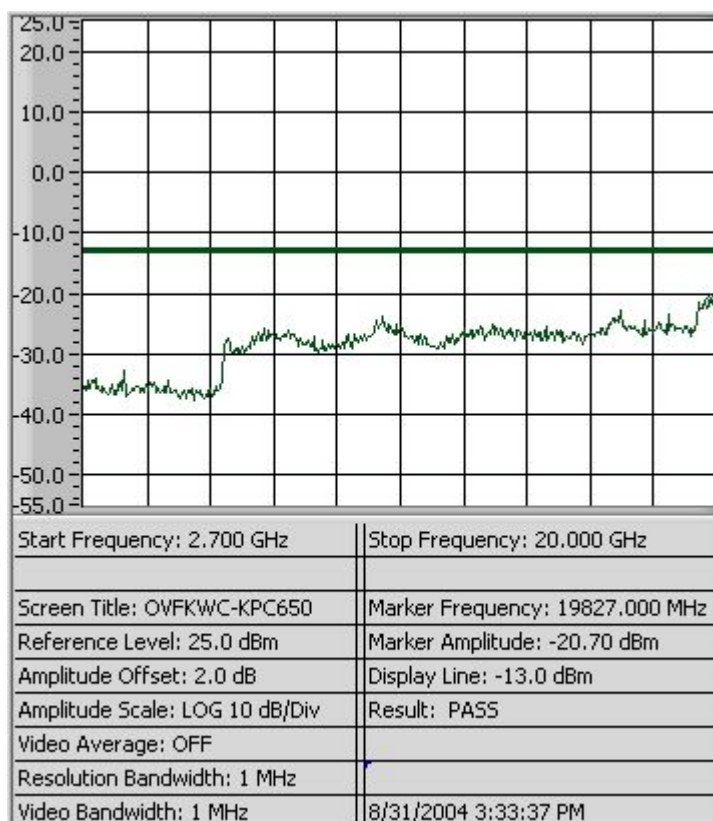
Figure 8-8b CDMA 1900 - Conducted Spurious Emission (CH 600)
