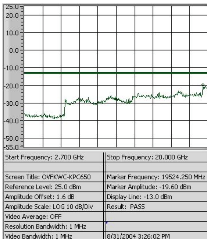
Figure 8-6b CDMA 800 – Conducted Spurious Emission (CH 777)
