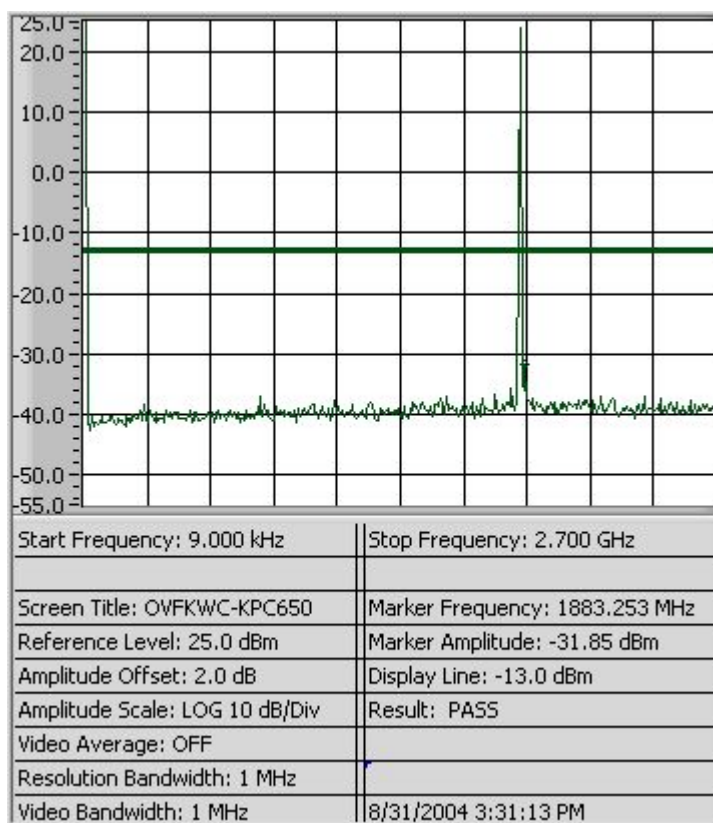
Figure 8-7a CDMA 1900 - Conducted Spurious Emission (CH 25)
