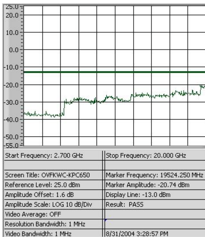
Figure 8-2b CDMA 800 – Conducted Spurious Emission (CH 1013)
