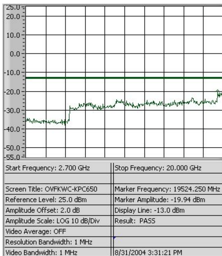
Figure 8-7b CDMA 1900 - Conducted Spurious Emission (CH 25)
