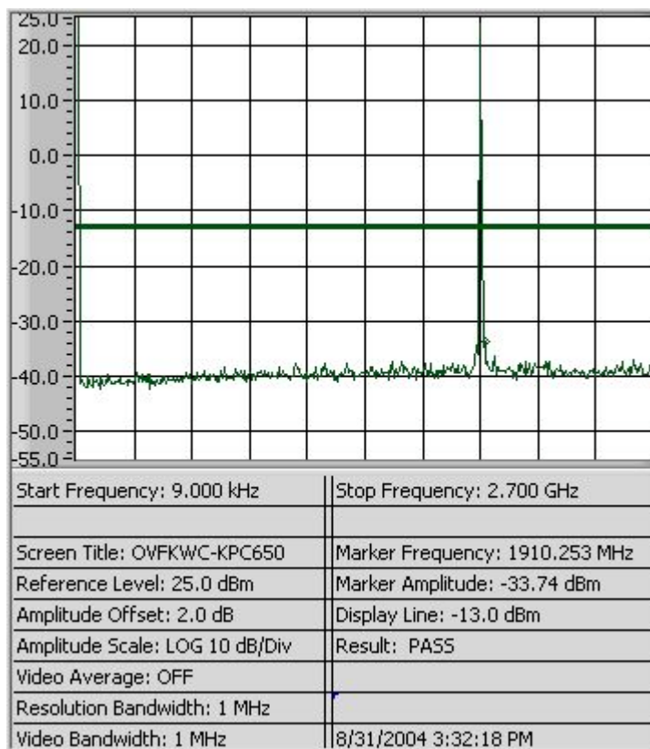
Figure 8-9a CDMA 1900 - Conducted Spurious Emission (CH 1175)
