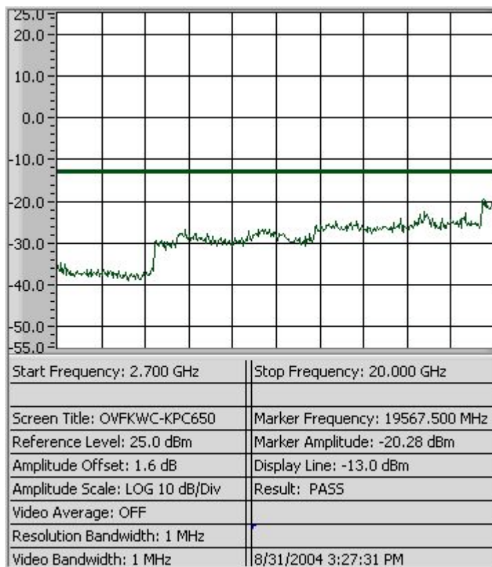
Figure 8-4b CDMA 800 – Conducted Spurious Emission (CH 383)
