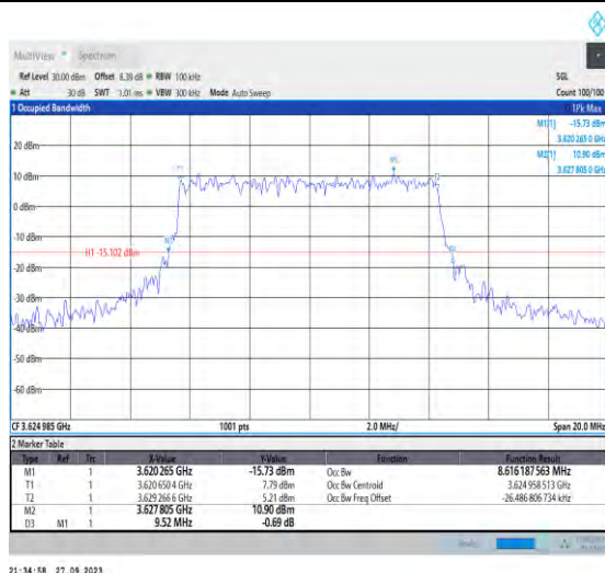
1-N48-PC3-30-10-M-3-DFT-16QAM-Outter_Full-24@0-Ant7-8.616-9.520-≤10-PASS
