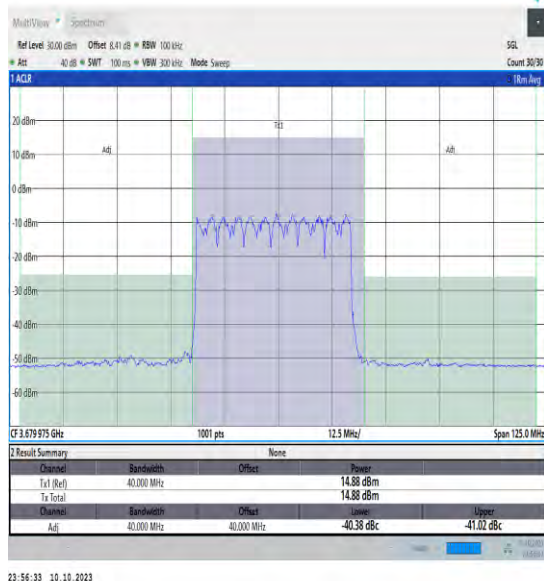
NTVN_N48_PC3_30_40_H_TID1_#1_-40_40
