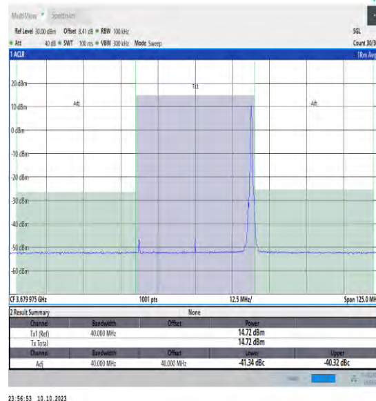
NTVN_N48_PC3_30_40_H_TID3_#1_-40_40
