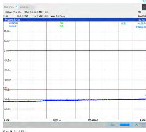
1-N48-PC3-30-40-H-1-DFT-PI2BPSK-Inner_1RB_Lef t-1@1-1000-3000-Ant7-2996.80--47.22--40-PASS
