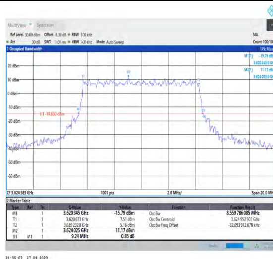
1-N48-PC3-30-10-M-4-DFT-64QAM-Outter_Full-24@0-Ant7-8.56-9.240-≤10-PASS
