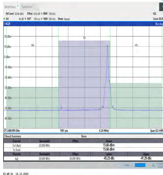
NTNV_N48_PC3_30_20_H_TID3_#1_-20_20
