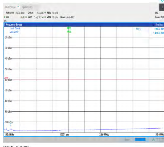
1-N48-PC3-30-40-H-1-DFT-PI2BPSK-Inner_1RB_Lef t-1@1-0.15-30-Ant7-0.15--87.60--60-PASS
