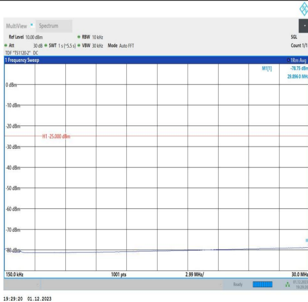
7-7-20MHz-15MHz-64QAM-64QAM-20850-21021-1RB#99-0R B#0-0.15~30MHz-PASS
