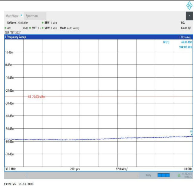
7-7-20MHz-15MHz-64QAM-64QAM-20850-21021-1RB#99-0R B#0-30~1000MHz-PASS
