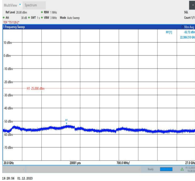
7-7-20MHz-15MHz-16QAM-16QAM-20850-21021-1RB#99-0R B#0-20000~27000MHz-PASS
