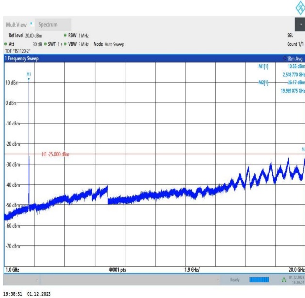
7-7-20MHz-15MHz-16QAM-16QAM-21026-21197-1RB#0-1RB #74-1000~20000MHz-PASS
