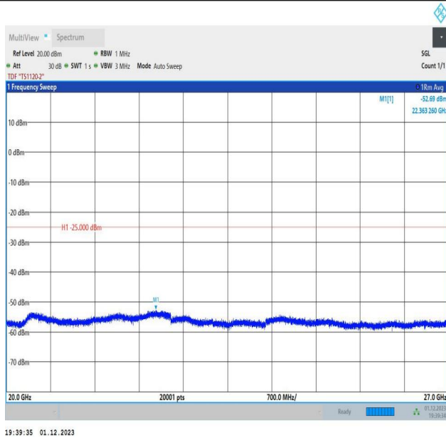
7-7-20MHz-15MHz-64QAM-64QAM-21026-21197-1RB#0-1RB #74-20000~27000MHz-PASS
