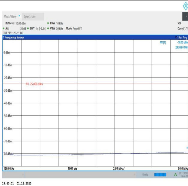
7-7-20MHz-15MHz-QPSK-QPSK-21026-21197-100RB#0-75R B#0-0.15~30MHz-PASS
