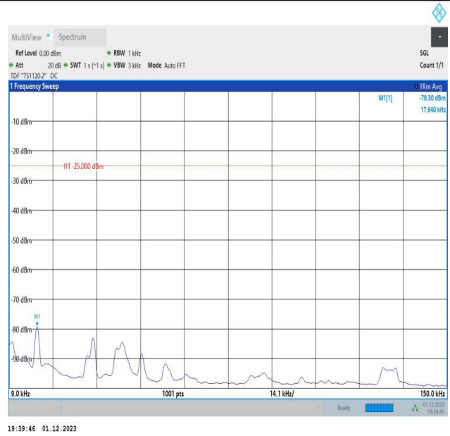
7-7-20MHz-15MHz-QPSK-QPSK-21026-21197-100RB#0-75R B#0-0.009~0.15MHz-PASS
