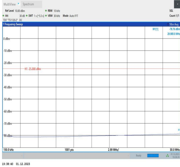
7-7-20MHz-15MHz-16QAM-16QAM-21026-21197-1RB#0-1RB #74-0.15~30MHz-PASS
