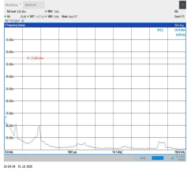
7-7-20MHz-15MHz-64QAM-64QAM-20850-21021-1RB#99-0R B#0-0.009~0.15MHz-PASS
