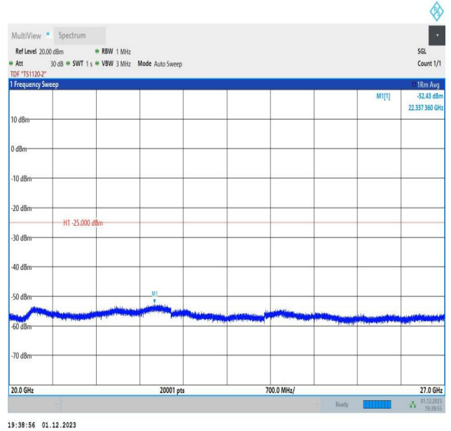
7-7-20MHz-15MHz-16QAM-16QAM-21026-21197-1RB#0-1RB #74-20000~27000MHz-PASS
