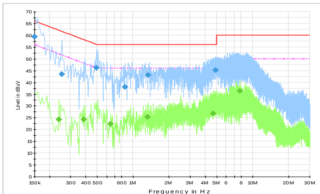
Fig.B.11.1 AC Powerline Conducted Emission- bluetooth
