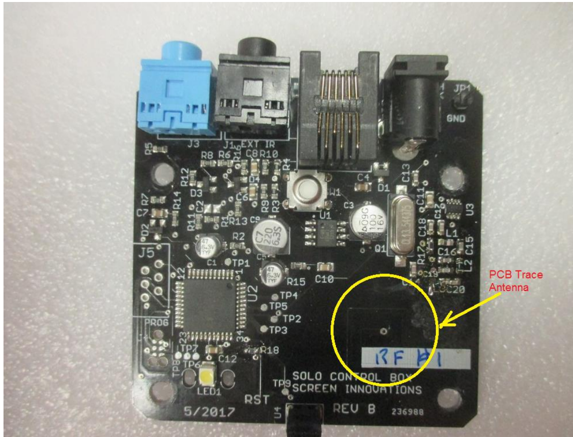
Figure 7.7 EUT PCB Component Side
