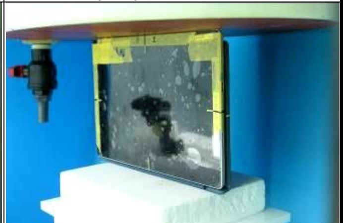
Body - Top Side of EUT at 0 mm w/ Keyboard
