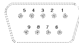
TELEMETERING SOCKET
