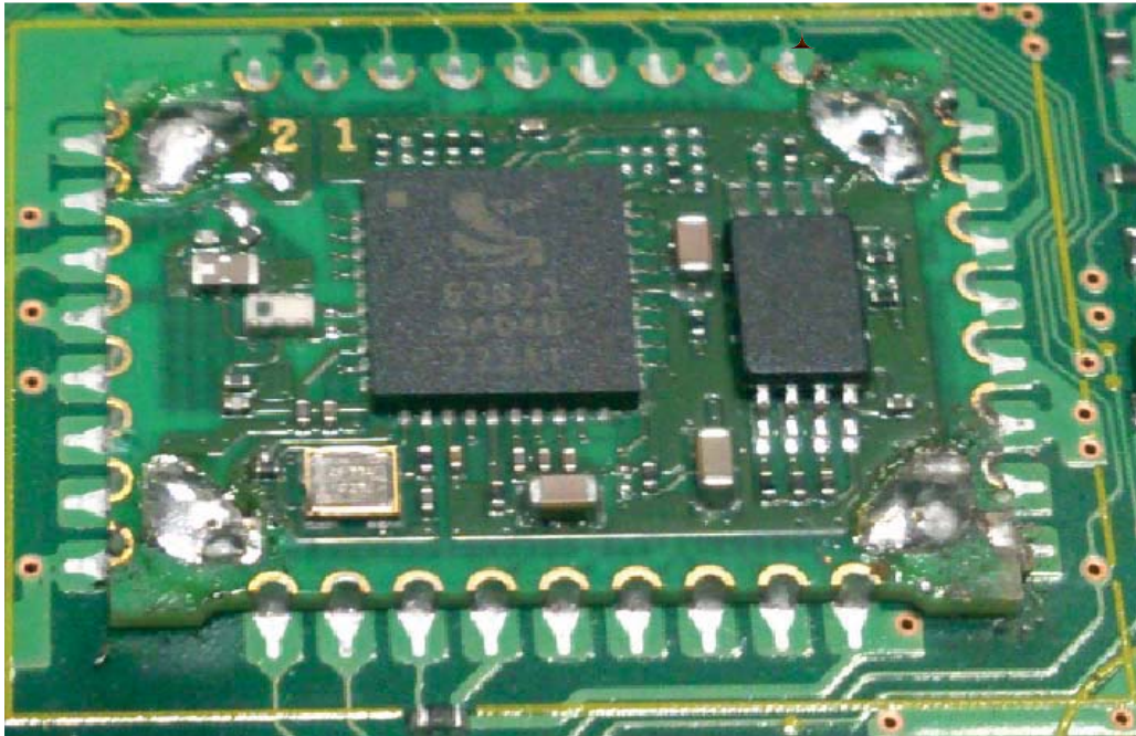
<Bluetooth part – without Shield>
