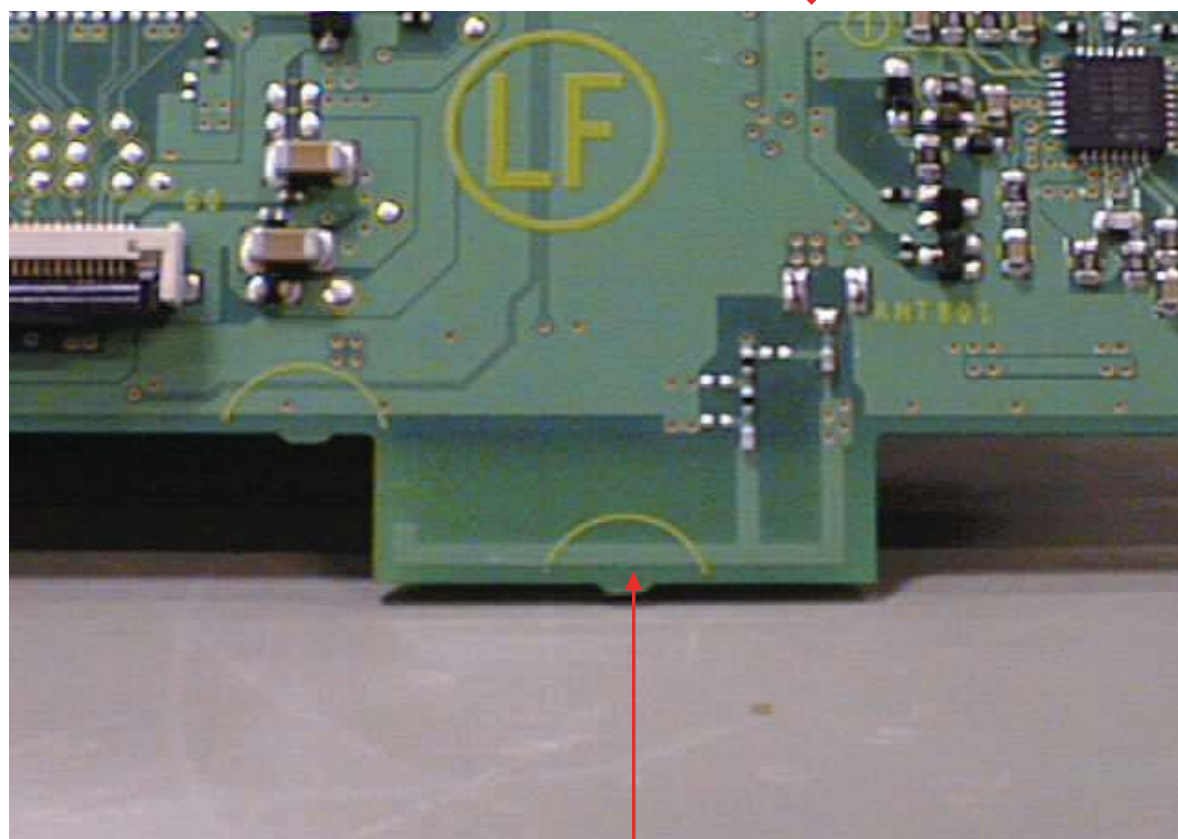
Bluetooth RF Antenna
