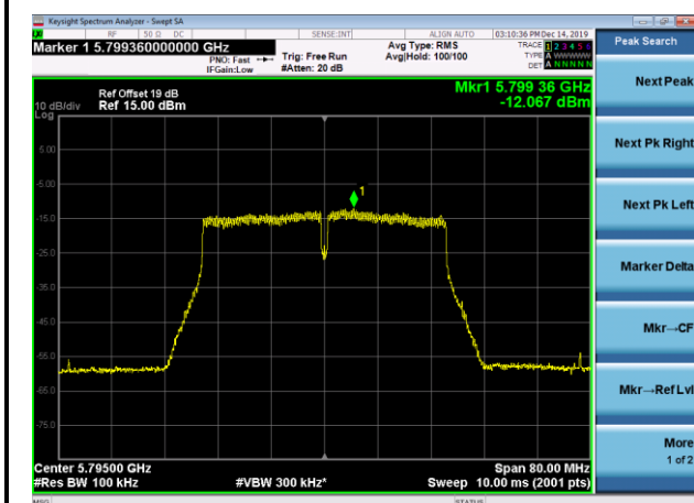
Channel 159 (5795MHz)
