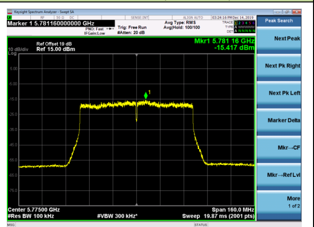
Channel 155 (5775MHz)
