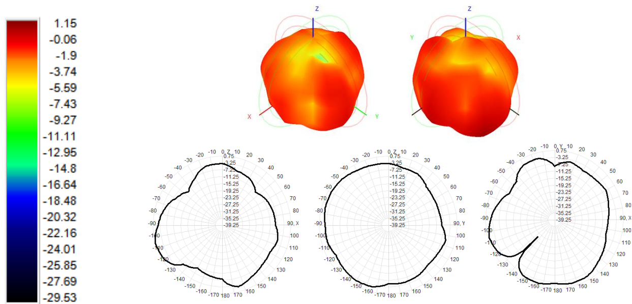
Passive field pattern diagram-2.4G
