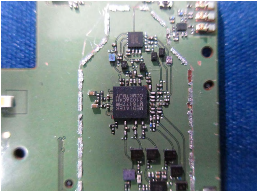
(22) EUT Photo
