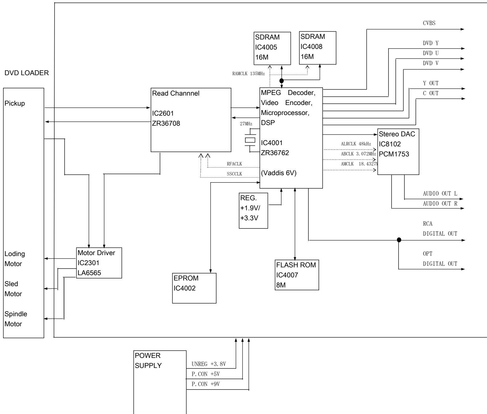
BLOCK DIAGRAM 2 (DVD Block)
