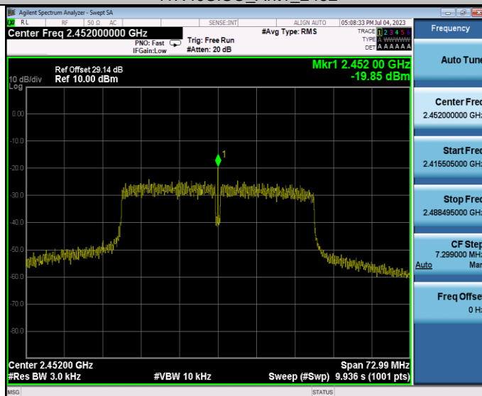
11N40SISO_Ant1_2452
