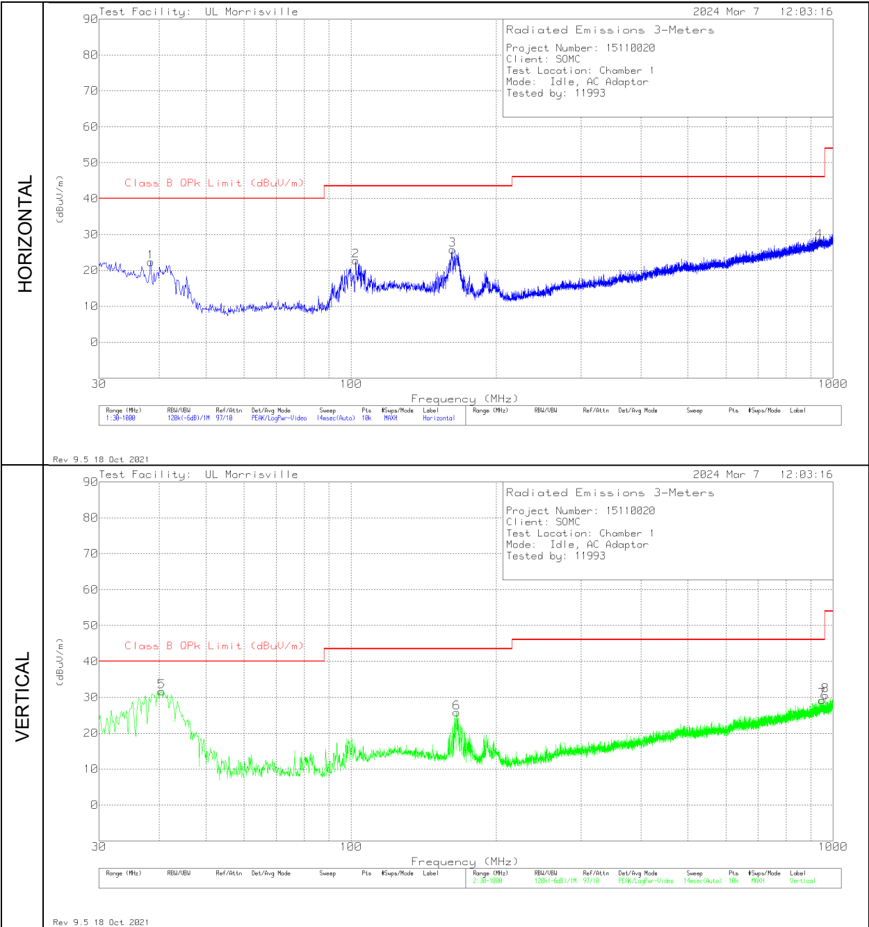
Radiated Emissions Graph
