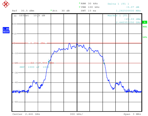
3DH1_Middle 1.283MHz
