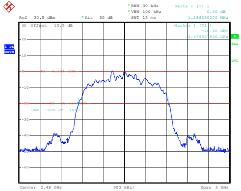
3DH1_High 1.286MHz
