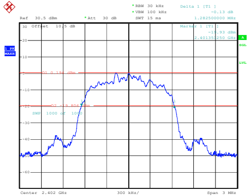
3DH1_Low 1.283MHz
