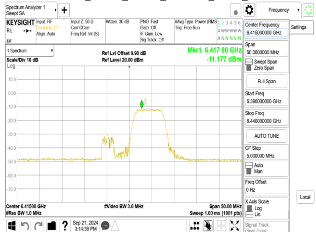
802.11be_20MHz_ChainA_6415MHz_RU106_54
