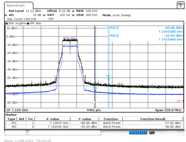
BE-NR-HIGH, SISO-B, 802.11ax/be20-MCS0, Ch229
