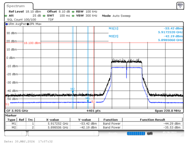
BE-NR-LOW, SISO-A, 802.11ax/be40-MCS0, Ch3
