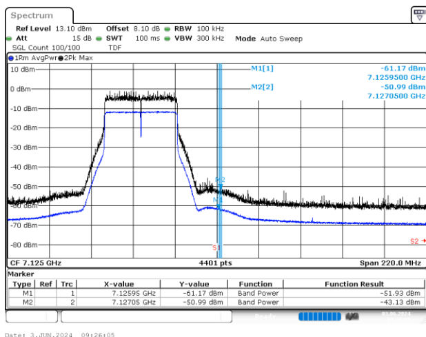
BE-NR-HIGH, SISO-B, 802.11ax/be40-MCS0, Ch227
