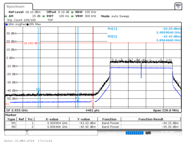
BE-NR-LOW, SISO-A, 802.11ax/be80-MCS0, Ch7
