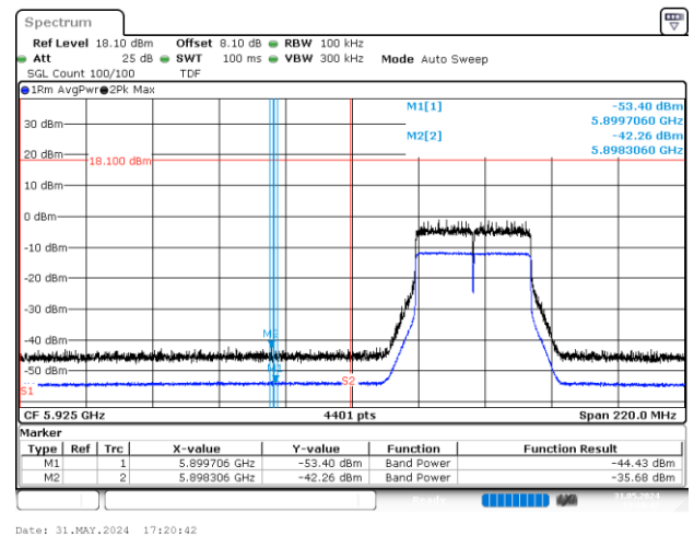
BE-NR-LOW, SISO-B, 802.11ax/be40-MCS0, Ch3
