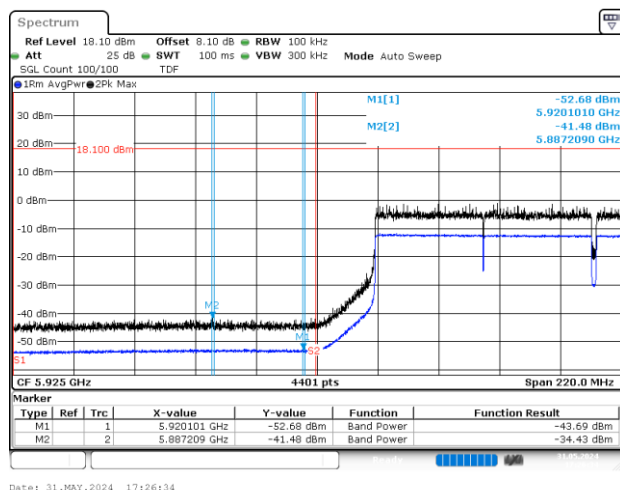
BE-NR-LOW, SISO-B, 802.11ax/be160-MCS0, Ch15
