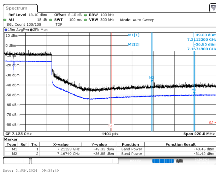
BE-NR-HIGH, SISO-B, 802.11be320-MCS0, Ch191
