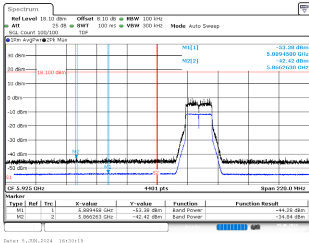
BE-NR-LOW, SISO-B, 802.11ax/be20-MCS0, Ch1
