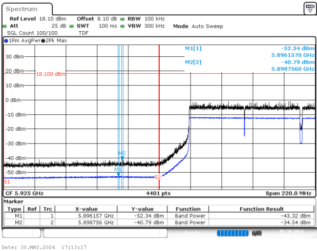
BE-NR-LOW, SISO-A, 802.11ax/be160-MCS0, Ch15
