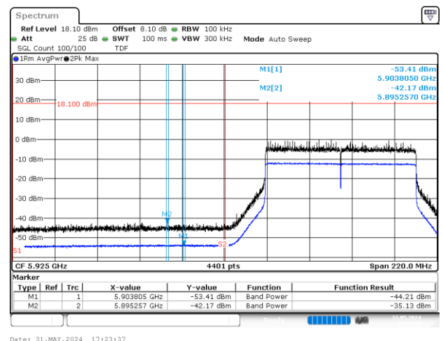
BE-NR-LOW, SISO-B, 802.11ax/be80-MCS0, Ch7
