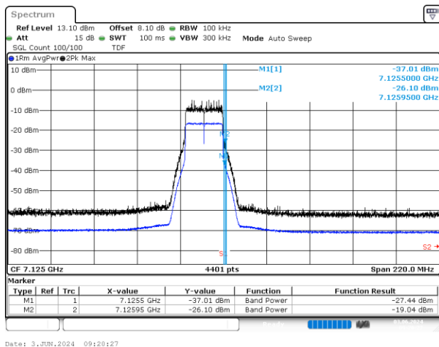
BE-NR-HIGH, SISO-B, 802.11ax/be20-MCS0, Ch233
