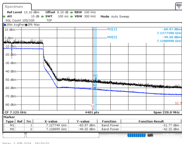
BE-NR-HIGH, SISO-B, 802.11ax/be80-MCS0, Ch215
