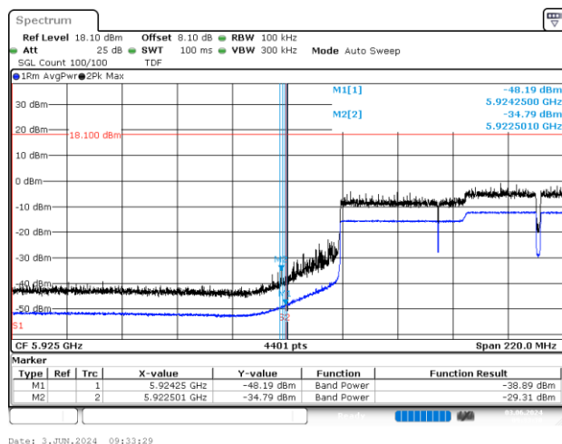
BE-NR-LOW, SISO-B, 802.11be320-MCS0, Ch31
