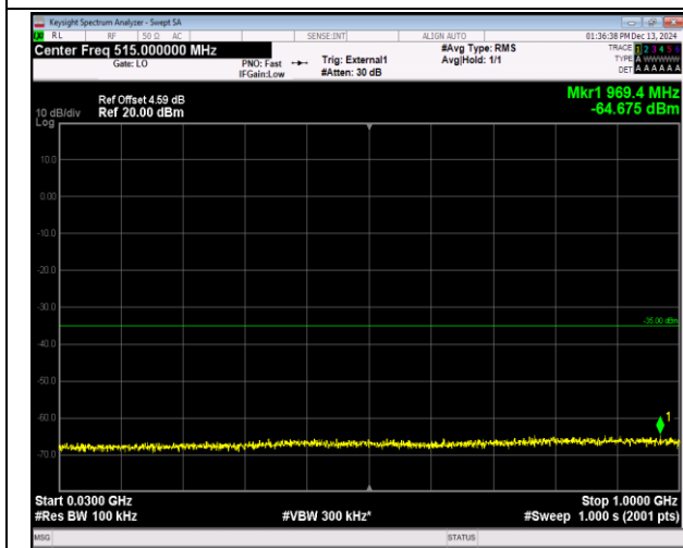
38-38-20MHz-20MHz-16QAM-16QAM-37850-38048-1RB #0-0RB#0-30~1000MHz-PASS
