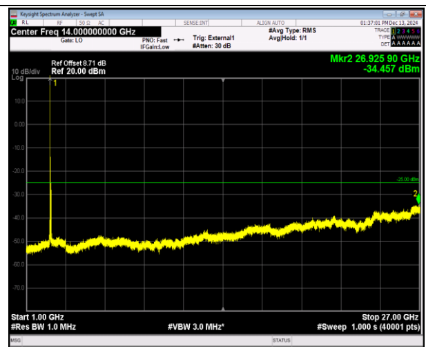
38-38-20MHz-20MHz-16QAM-16QAM-37850-38048-1RB#0-0RB#0-1000~27000MHz-PASS
