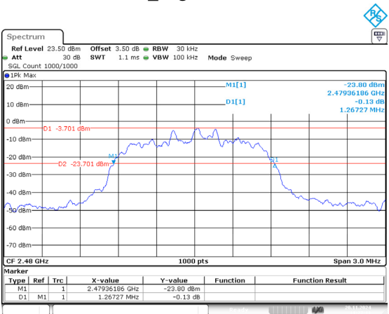
2DH1_High 1.267MHz
