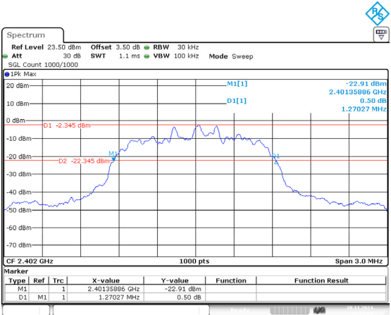
2DH1_Low 1.270MHz
