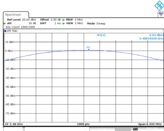
2DH1_High 0.65dBm
