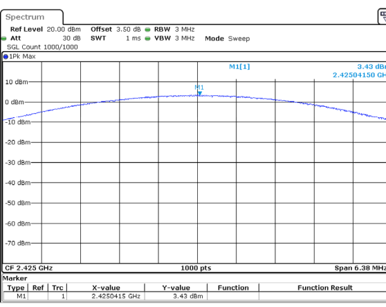
3DH1_Additional 3.43dBm
