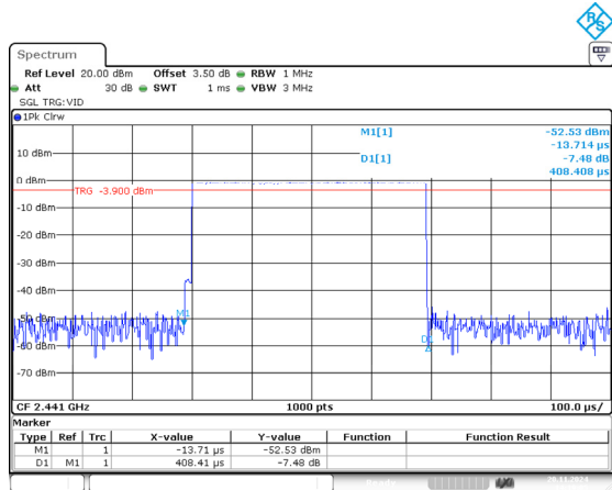
DH1_Hopping 0.408ms
