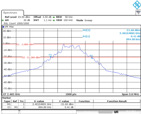
DH1_Low 0.895MHz
