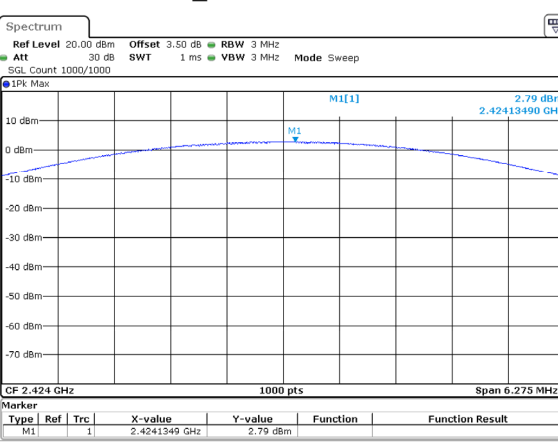
2DH1_Additional 2.79dBm
