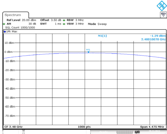
DH1_High -1.29dBm
