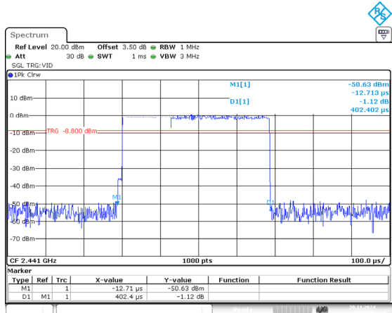
2DH1_Hopping 0.402ms
