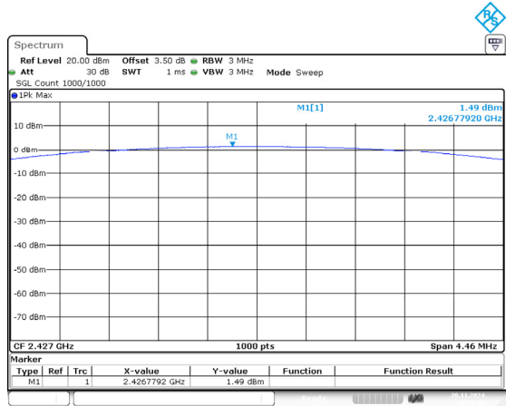
DH1_Additional 1.49dBm
