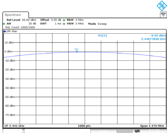
DH1_Middle -0.92dBm
