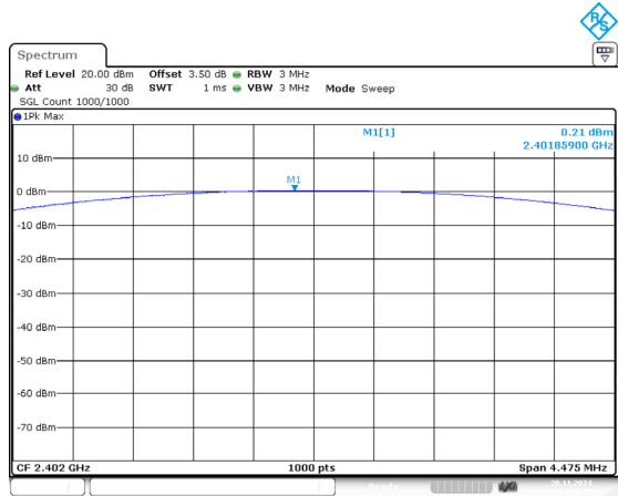
DH1_Low 0.21dBm
