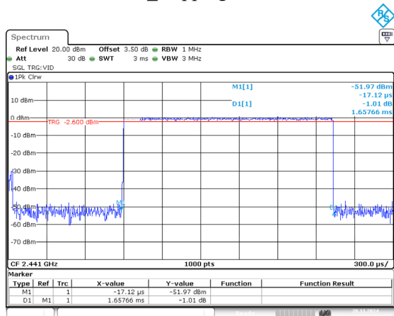
2DH3_Hopping 1.658ms
