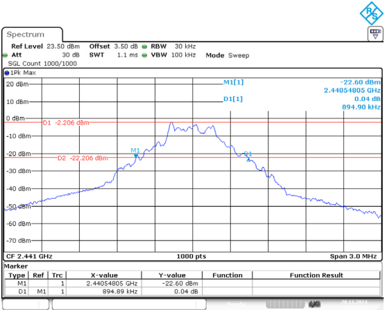
DH1_Middle 0.895MHz
