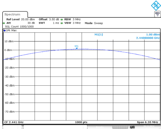
2DH1_Middle 1.00dBm
