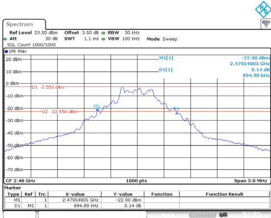
DH1_High 0.895MHz
