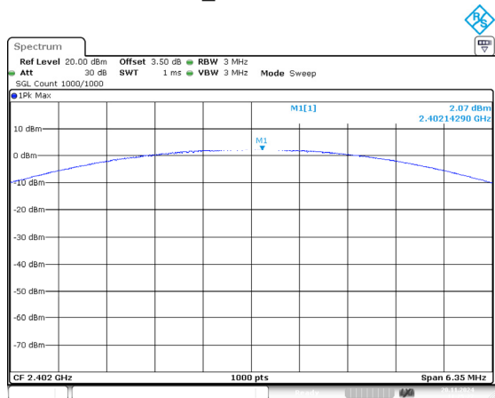
2DH1_Low 2.07dBm
