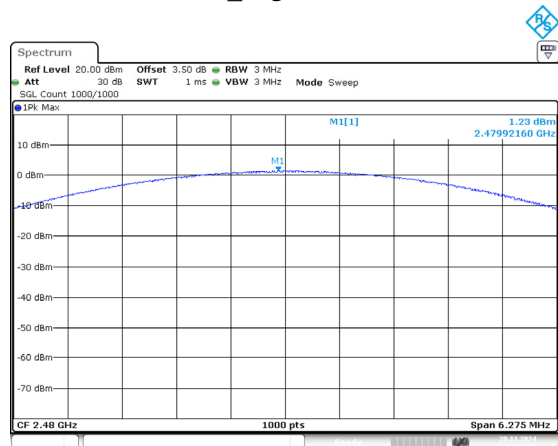
3DH1_High 1.23dBm
