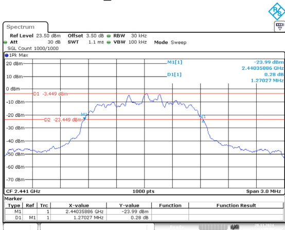
2DH1_Middle 1.270MHz
