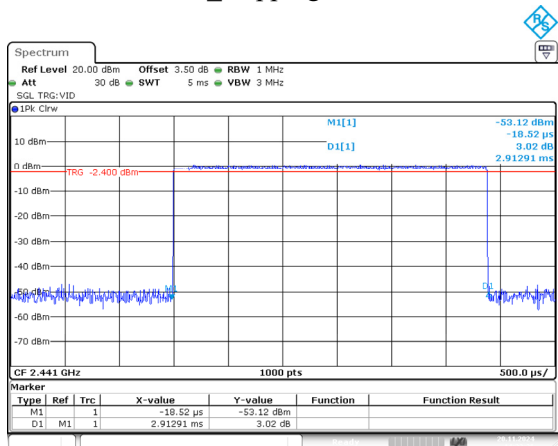
2DH5_Hopping 2.913ms
