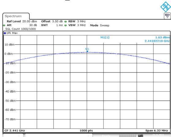
3DH1_Middle 1.63dBm
