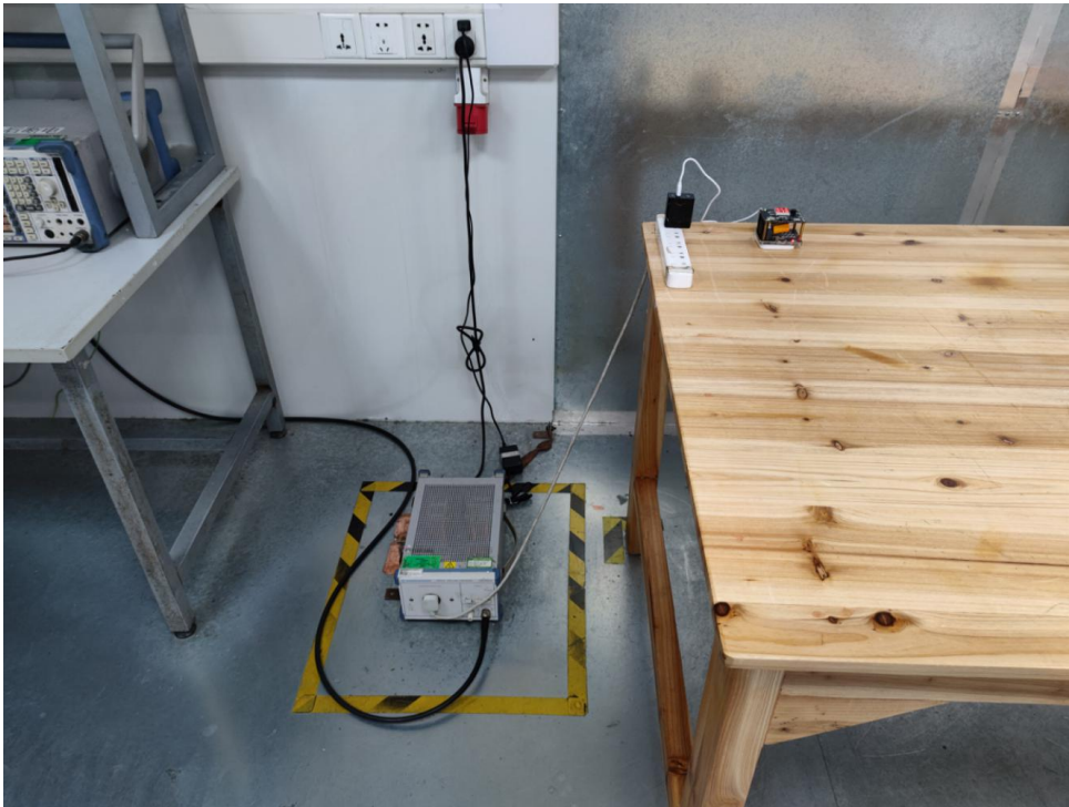
FCC ID: 2APU5-WPC380A Photo of Conducted Emission Measurement
