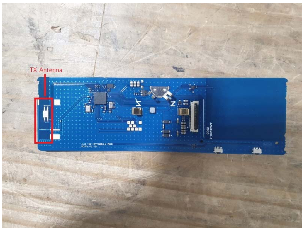
TX, RX Antenna
