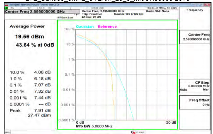
LTE_Band38_5MHz_64QAM_25_0_MidCH38000-2595
