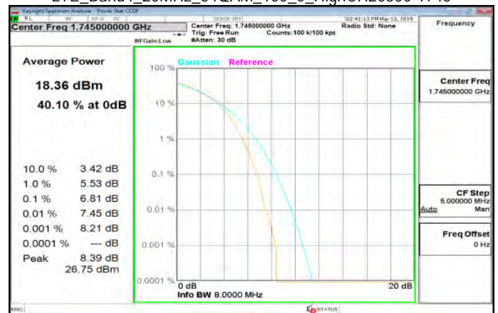
LTE_Band4_20MHz_64QAM_100_0_HighCH20300-1745
