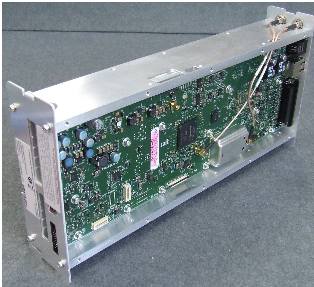
Photograph 02: Reciter module – Internal (Control PCB side)
