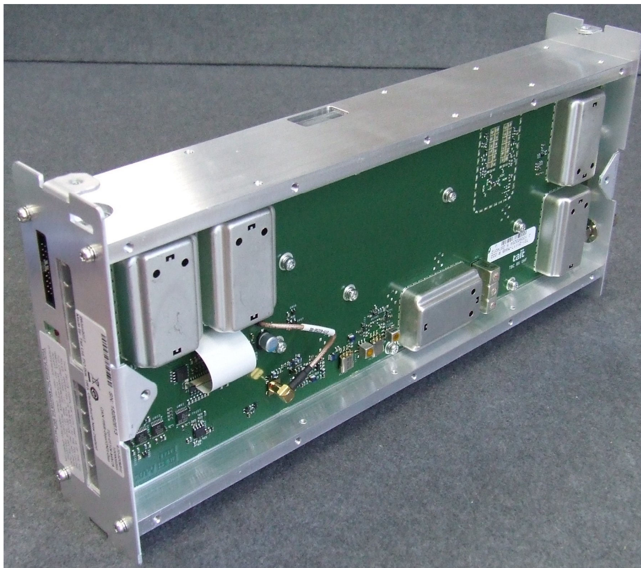
Photograph 01: Reciter module – Internal (Receiver PCB side)
