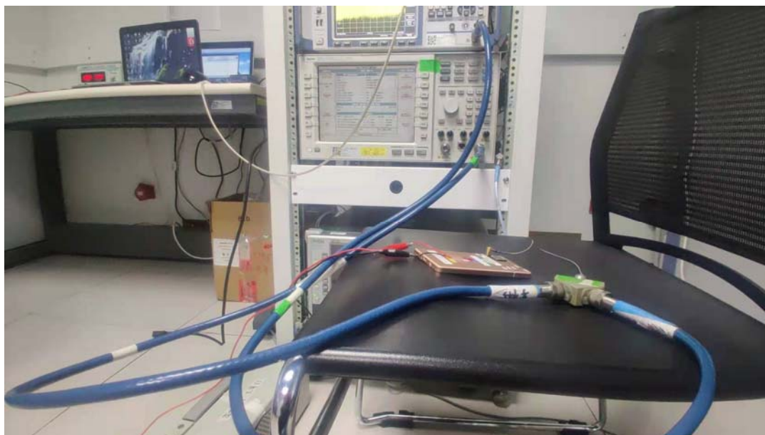
RF Conducted Test setup (GSM/WCDMA/LTE)
