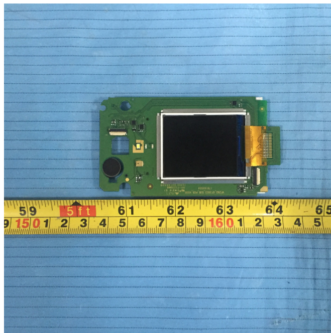
EUT – LCD Board Bottom View 1
