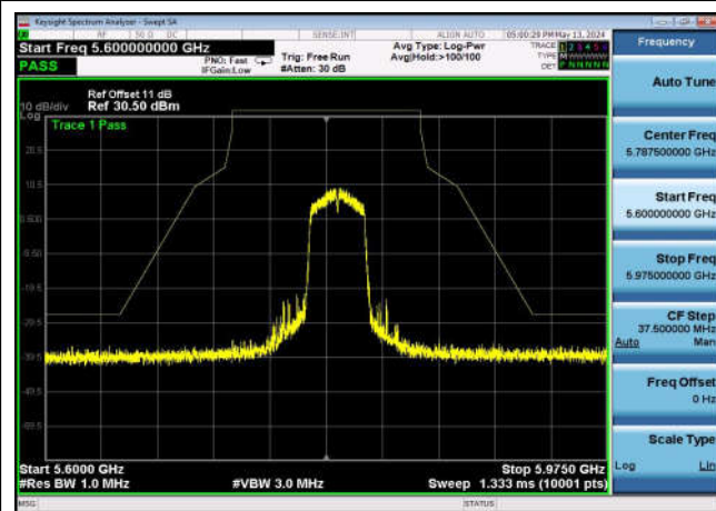
U-NII-3 ,Plot 1,Band Edge-802.11n(40M Hz),5795MHz,Ant0
