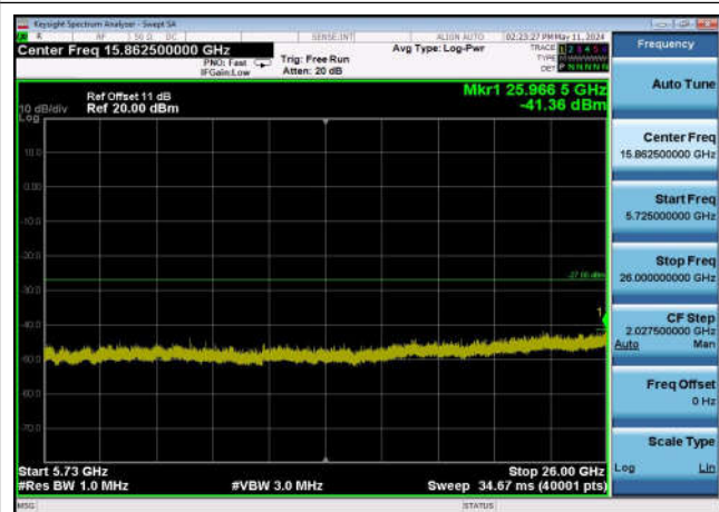
U-NII-2c ,Plot 3,5725MHz~26000MHz-802 .11a(20MHz),5500MHz,Ant0
