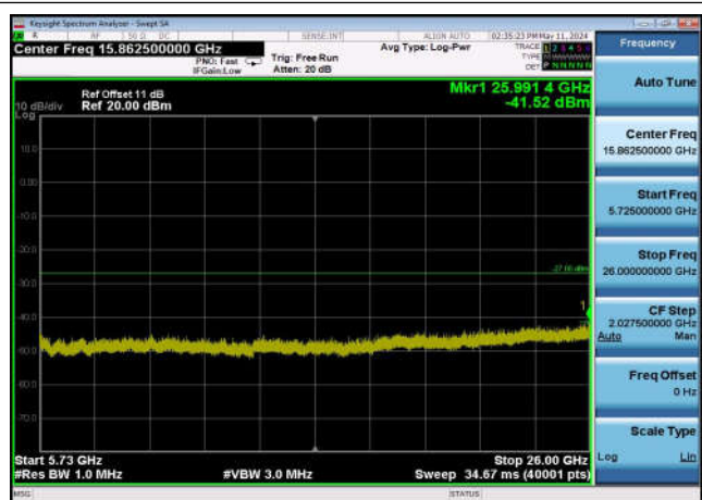
U-NII-2c ,Plot 3,5725MHz~26000MHz-802 .11a(20MHz),5600MHz,Ant0
