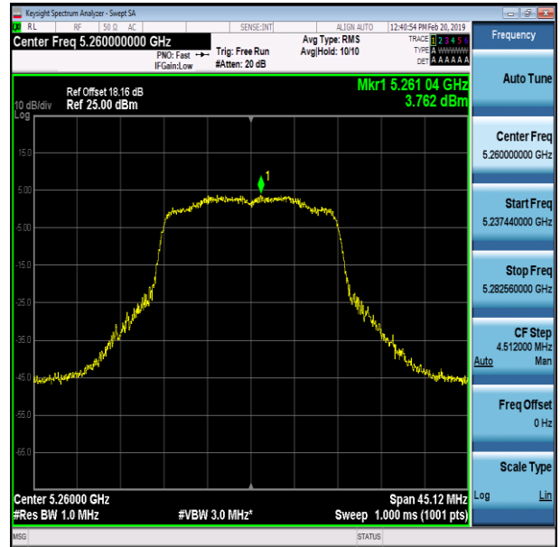
11AC20SISO-Ant1-5260
