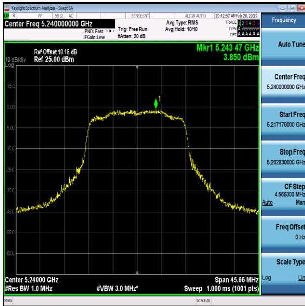
11N20SISO-Ant1-5240
