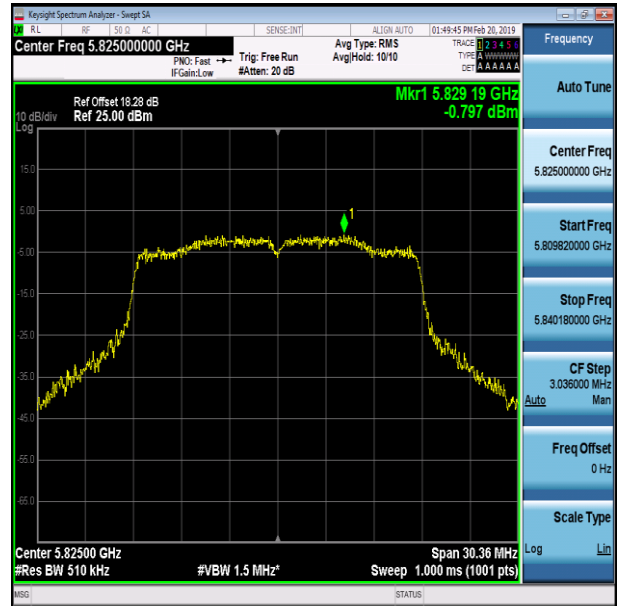
11AC20SISO-Ant1-5825
