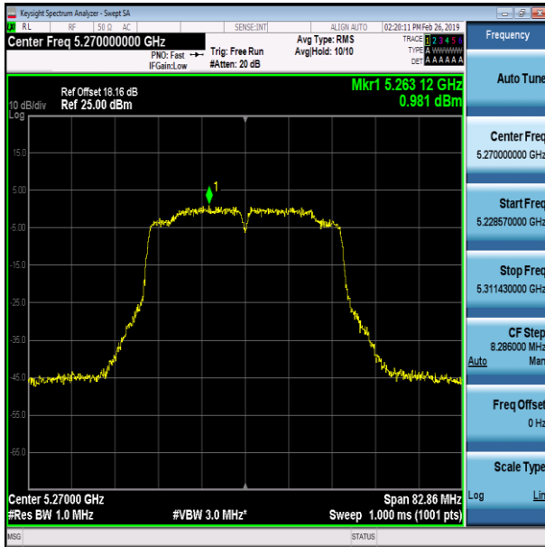
11AC40SISO-Ant1-5270
