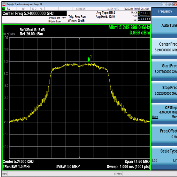
11AC20SISO-Ant1-5240
