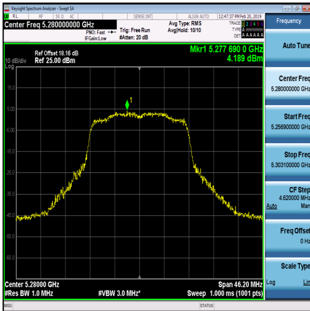
11AC20SISO-Ant1-5280
