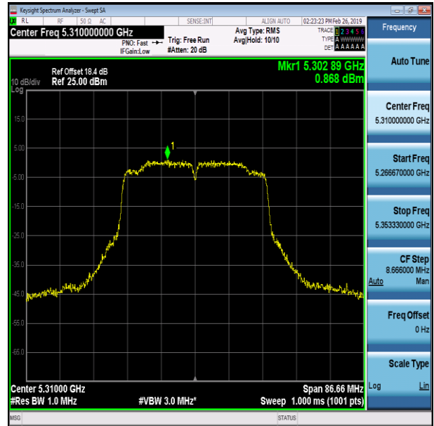
11AC40SISO-Ant1-5310
