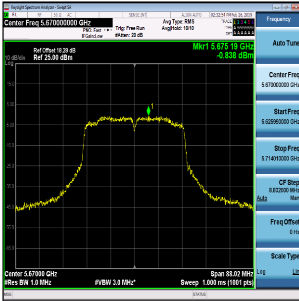
11AC40SISO-Ant1-5670
