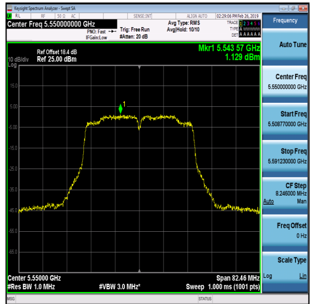
11AC40SISO-Ant1-5550
