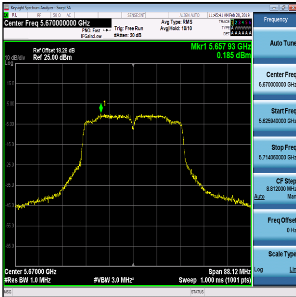
11N40SISO-Ant1-5670
