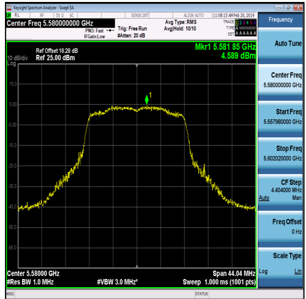
11N20SISO-Ant1-5580
