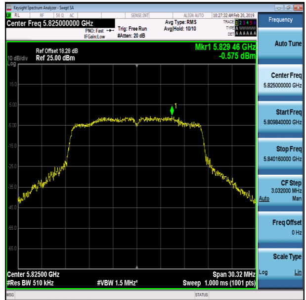
11A-Ant1-5825
