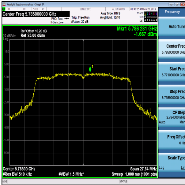
11AC20SISO-Ant1-5785
