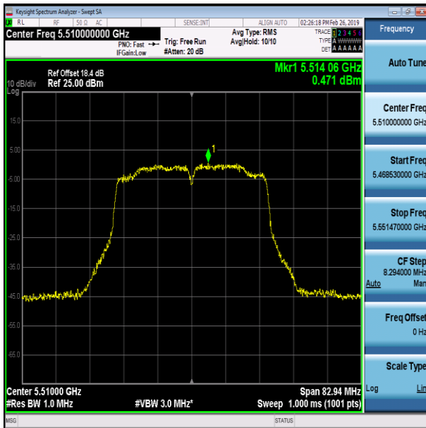
11AC40SISO-Ant1-5510
