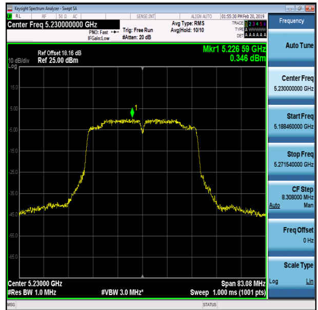
11AC40SISO-Ant1-5230
