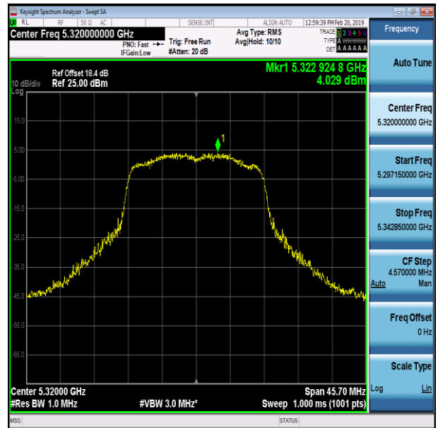
11AC20SISO-Ant1-5320
