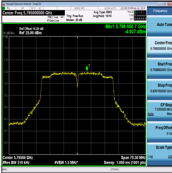
11AC40SISO-Ant1-5795
