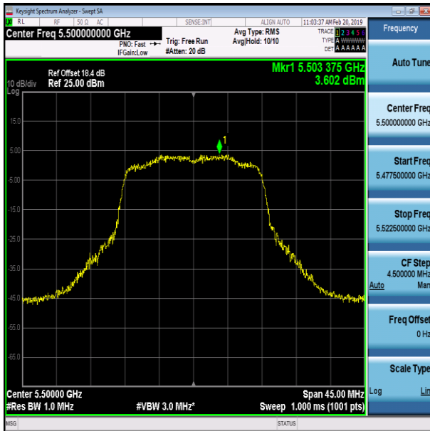
11N20SISO-Ant1-5500
