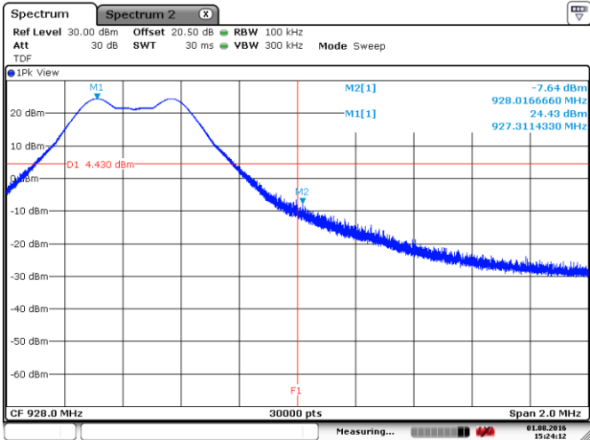
Figure 8.4-11: Upper band edge emission, tx on high channel
