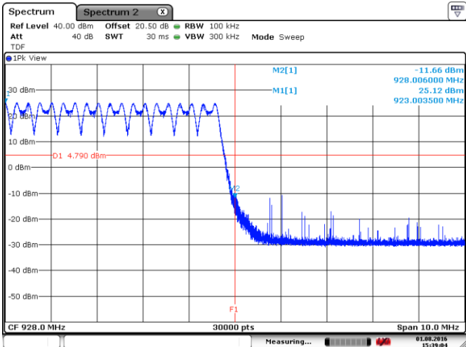
Figure 8.4-13: Upper band edge emission, tx hopping on
