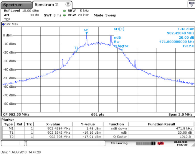
Figure 8.2-1: 20 dB bandwidth on low channel
