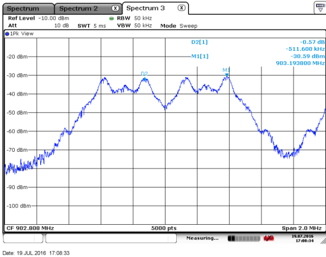
Figure 8.2-4: Carrier frequency separation
