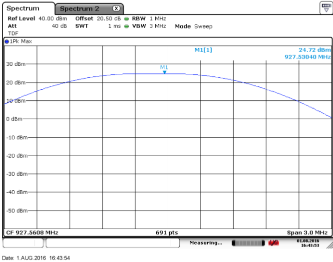
Figure 8.3-3: Output power on high channel, 102 V AC
