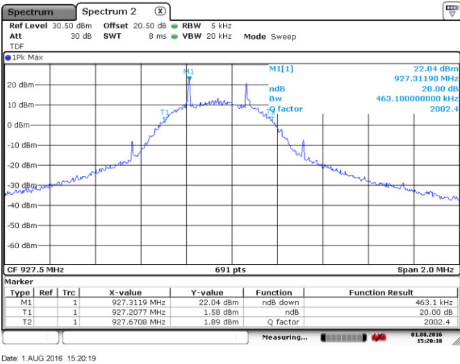
Figure 8.2-3: 20 dB bandwidth on high channel
