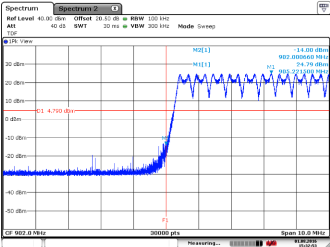
Figure 8.4-12: Lower band edge emission, tx hopping on
