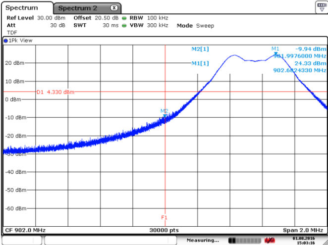
Figure 8.4-10: Lower band edge emission, tx on low channel
