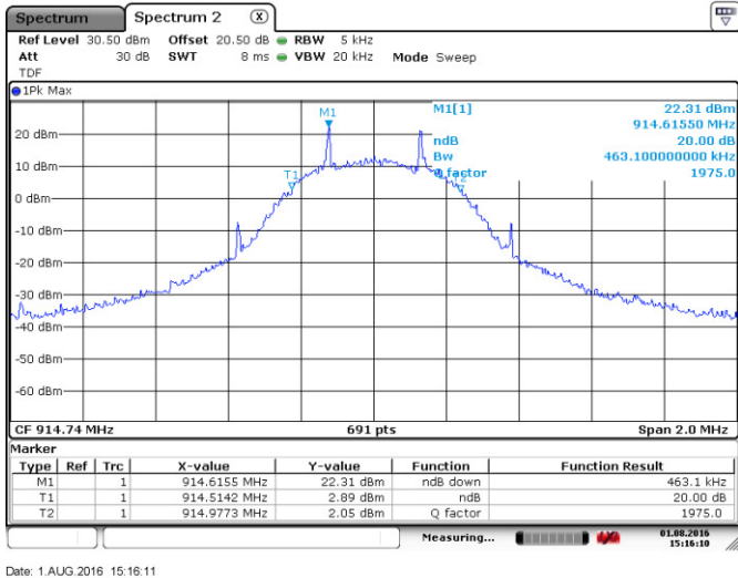
Figure 8.2-2: 20 dB bandwidth on mid channel
