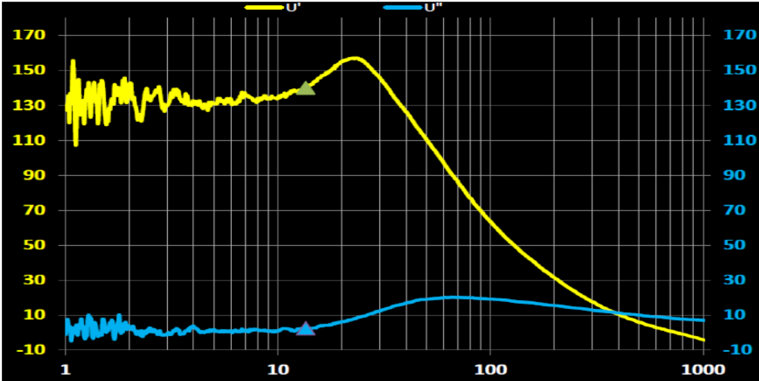
Permeability
