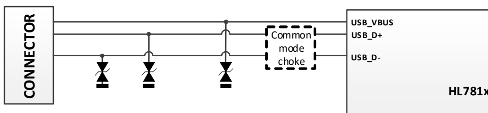
Figure 6-2: ESD Suppressors for USB FS
