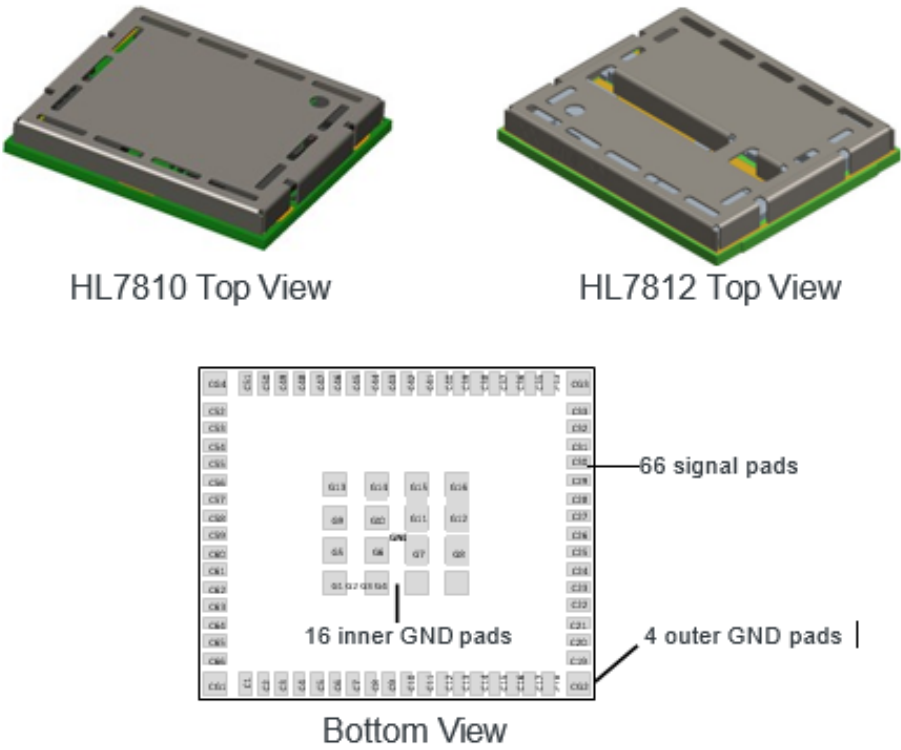
Figure 1-1: Mechanical Overview
