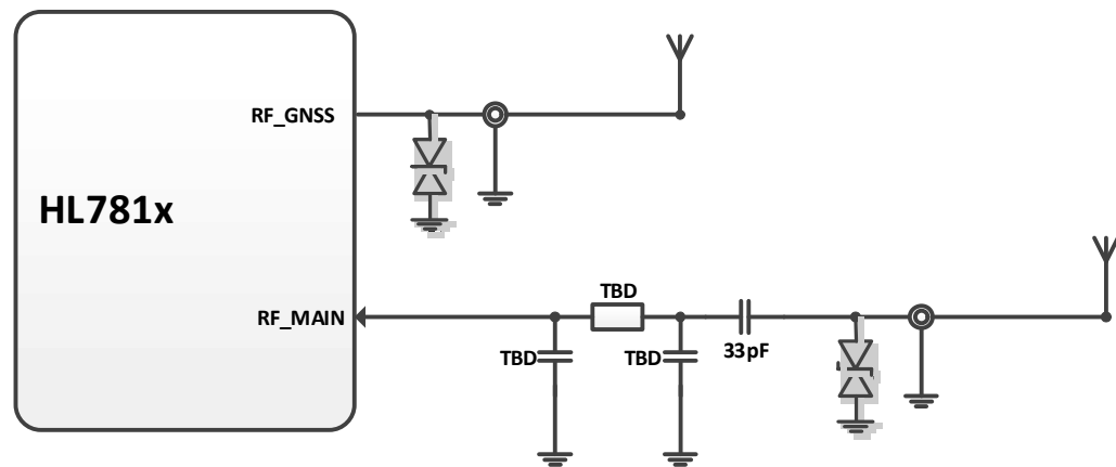
Figure 6-5: Antenna Connection
