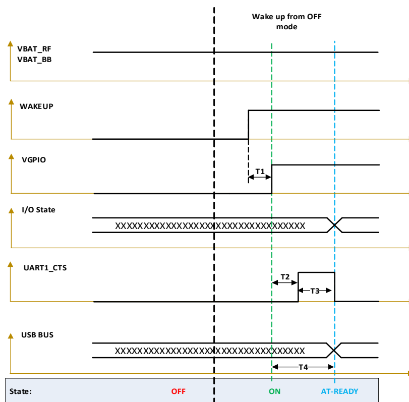
Figure 4-7: Wake up from OFF Mode
