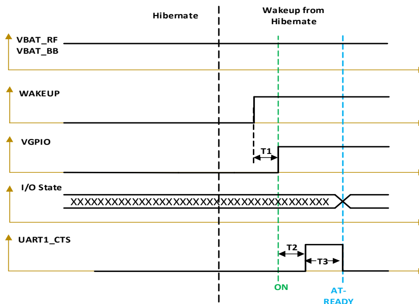
Figure 4-9: Wake up from Hibernate Mode
