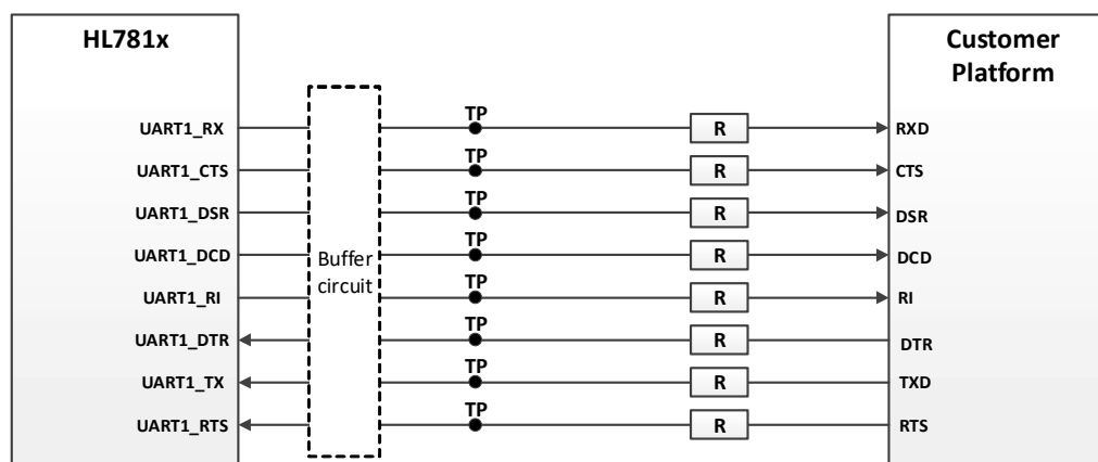
Figure 4-1: 8-wire UART Application Example
