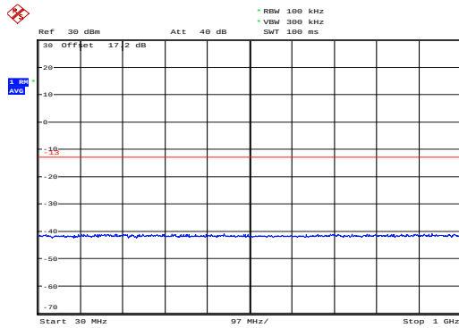
LTE Band 4 1.4MHz CH-Low 30MHz~1GHz
