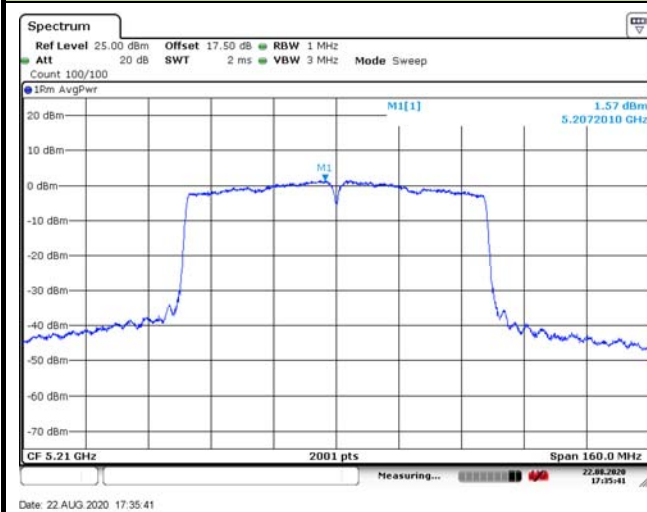
Channel 42 (5210MHz)
