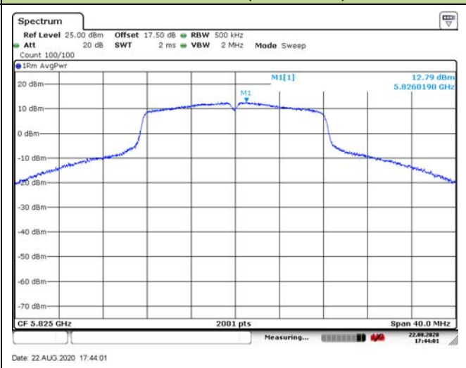
Channel 165 (5825MHz)
