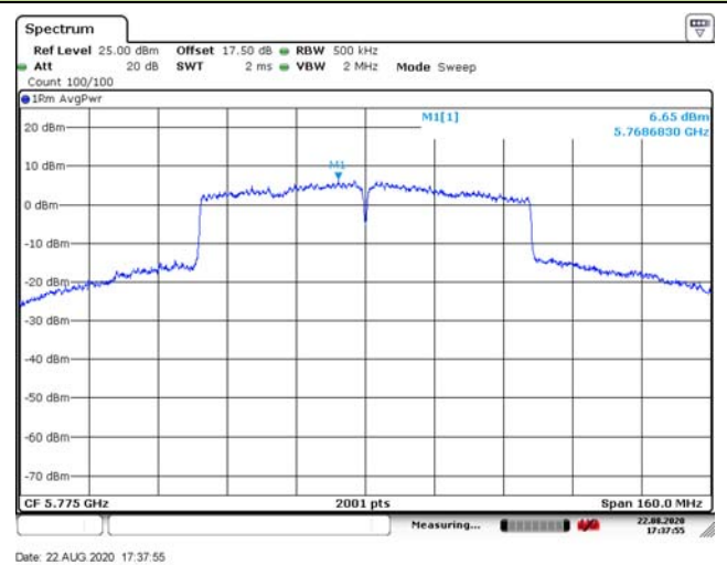
Channel 155 (5775MHz)
