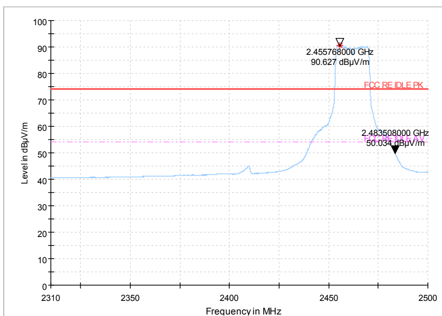
Fig 63. Radiated emission (Power): 802.11g, high channel
