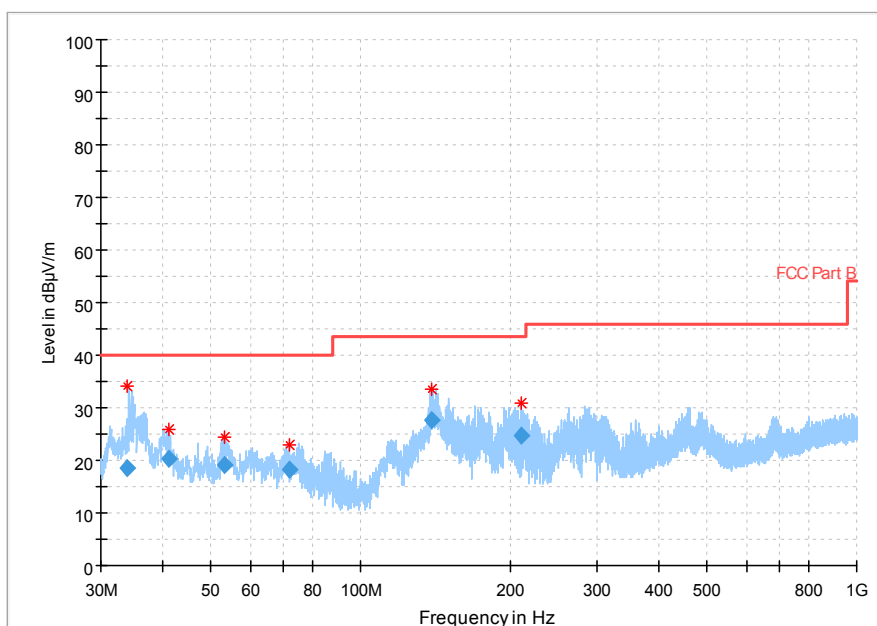
Fig 74. Radiated Spurious Emission (802.11 n-40MHz, Ch3, 30MHz~1GHz)
