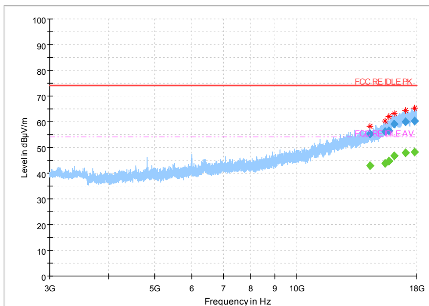
Fig 81. Radiated Spurious Emission (802.11b, Ch1, 3GHz~18GHz)
