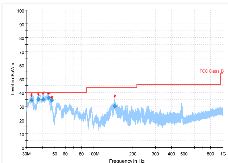
Fig 79. Radiated Spurious Emission (802.11b, Ch1,30MHz~1GHz)
