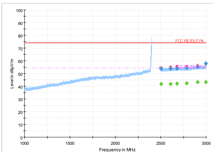
Fig 75. Radiated Spurious Emission (802.11 n-40MHz, Ch3, 1GHz~3GHz)
