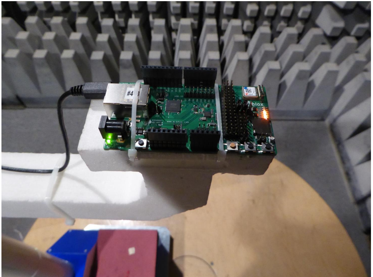
170297_E6_02.jpg: Test setup fully anechoic chamber
