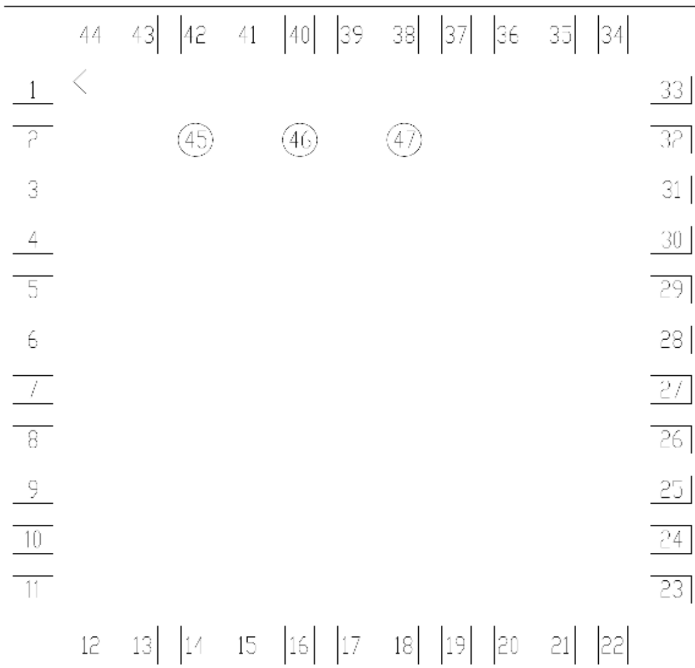
AW-NM512 Pin Map (Top View)
