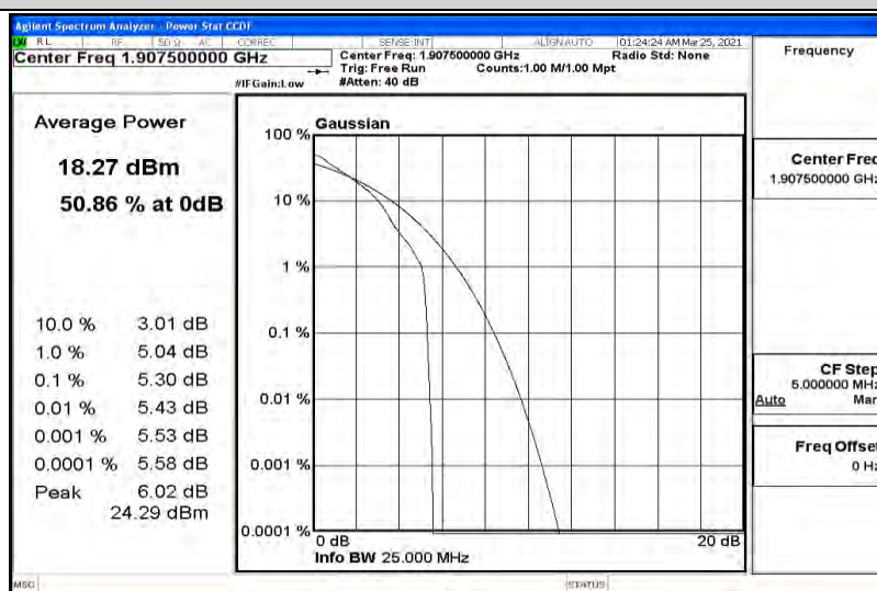
Band25-15MHz-QPSK-26615-75RB#0
