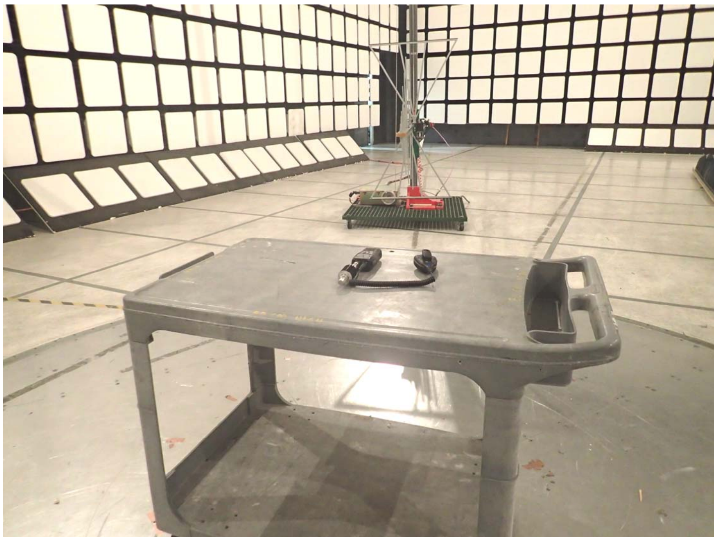
Radiated Emission at 3m (Orthogonal Position 1)
