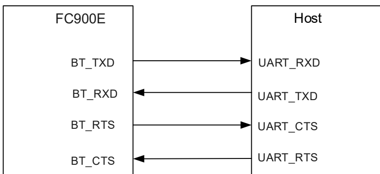
Figure 8: Reference Design for UART Interface Connection
