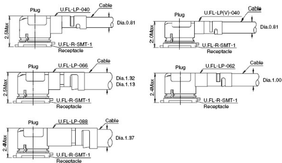
Figure 17: Space Factor of Mated Connectors (Unit: mm)
