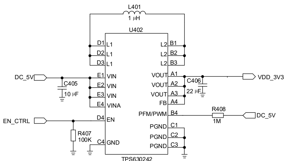
Figure 3: VBAT Circuit
