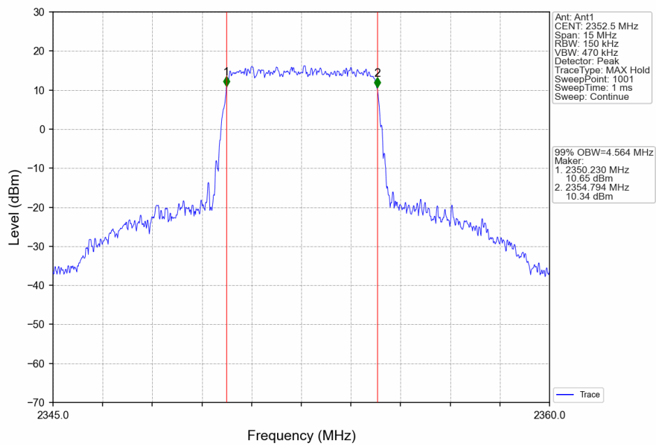
Band40b 5MHz 16QAM LCH 2352.5MHz RB 25 0 NTN
