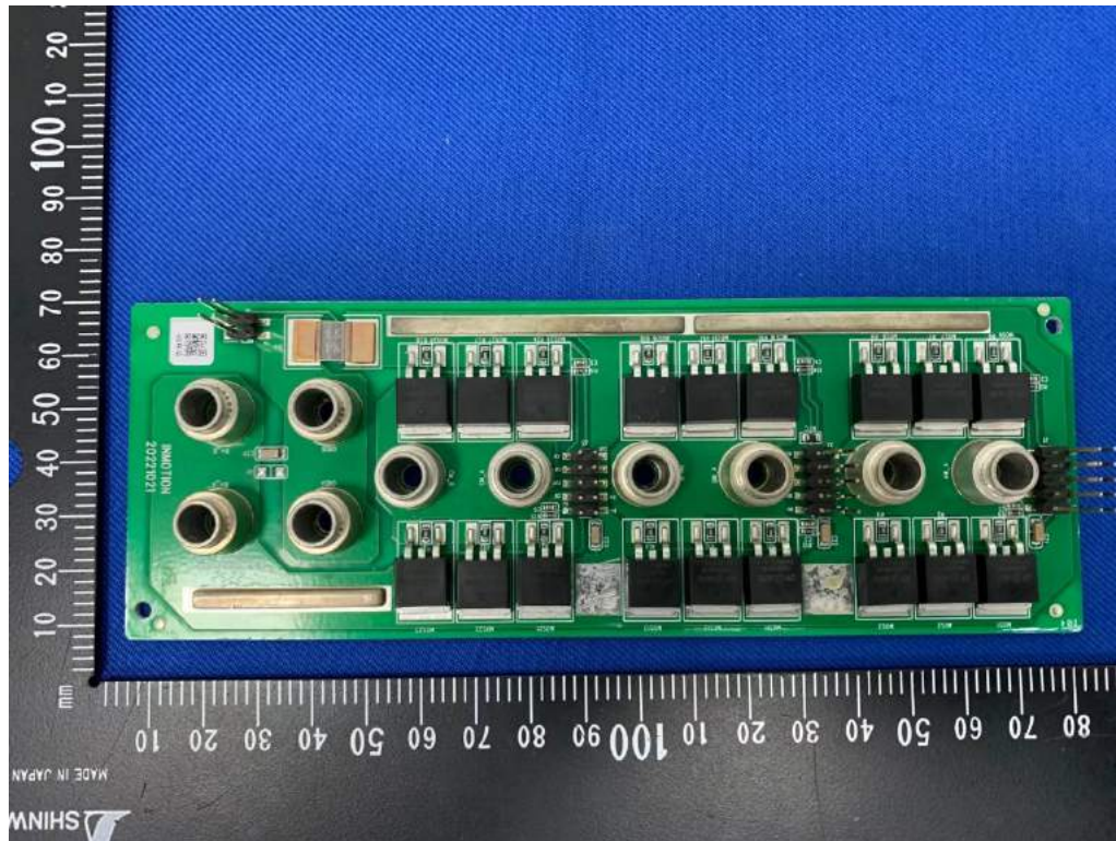
SUB BOARD TOP VIEW
