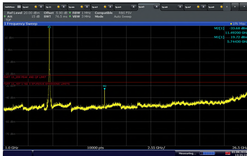
802.11 n (20 MHz) U-NII 3 Low Channel above 1GHz
