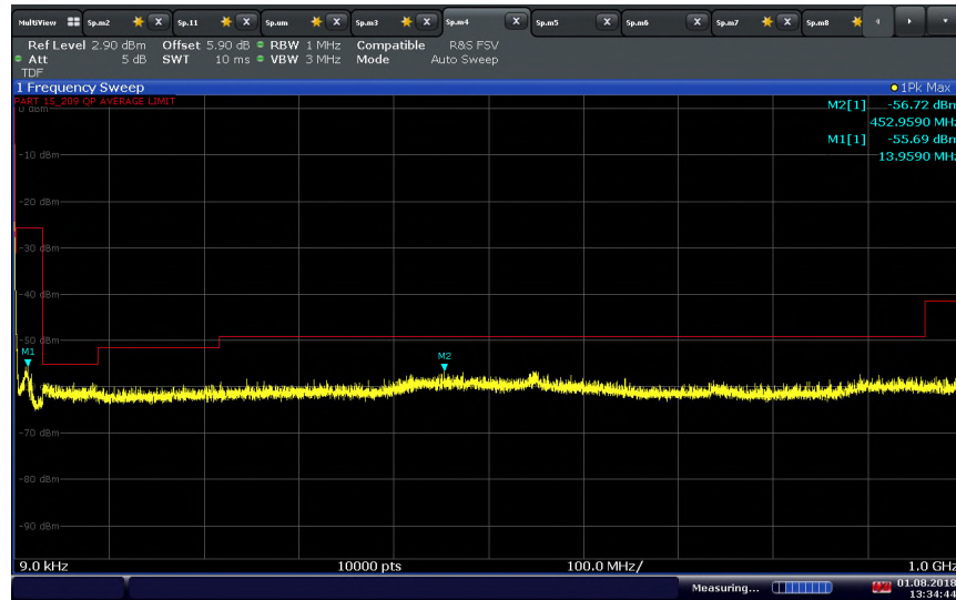
802.11 n (20 MHz) U-NII 3 Low Channel below 1GHz
