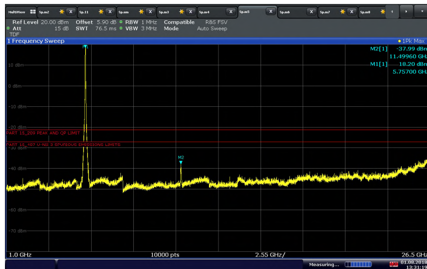
802.11 n (40 MHz) U-NII 3 Low Channel above 1GHz
