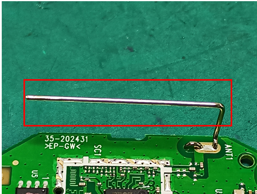
DECT ANT
