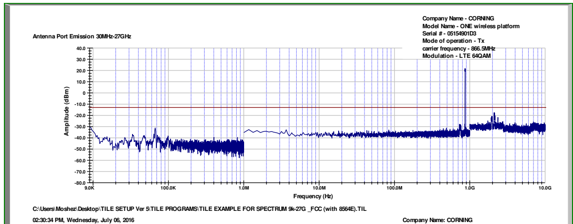
Figure 84. — 866.5 LTE 64QAM
