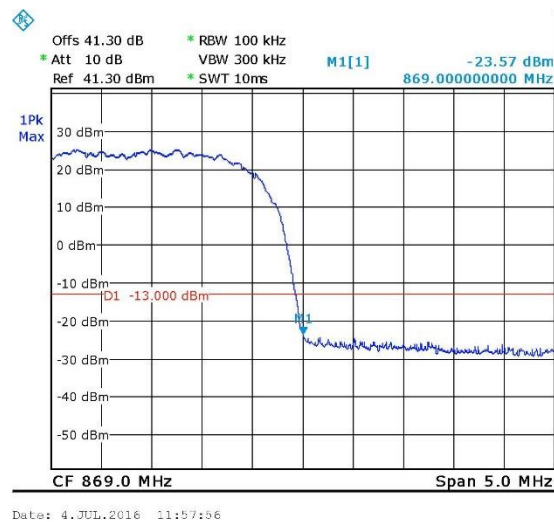
Figure 96. — W-CDMA - 866.5 MHz
