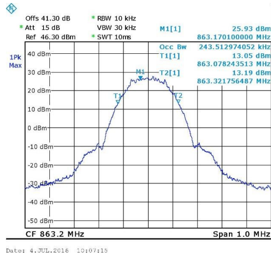
Figure 79. — 863.2MHz GSM Output
