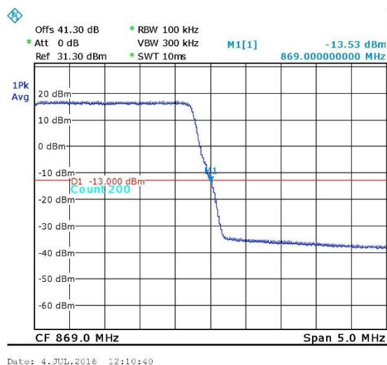
Figure 92. — LTE 64QAM 866.5 MHz
