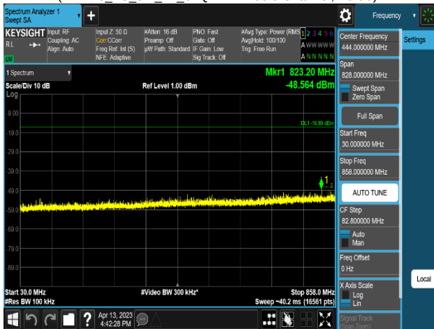
Plot 8-425. Conducted Spurious Emission Plot 30 MHz to 858 MHz (LTE B5_1C_5M_2T_64QAM - Middle Channel, Port 0)
