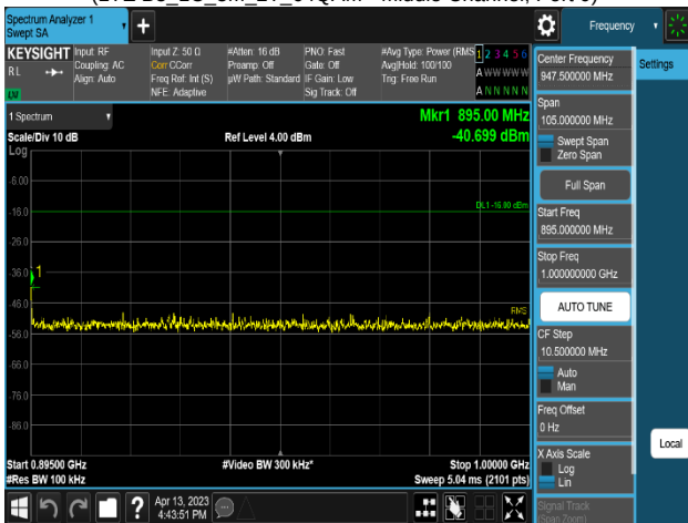
Plot 8-427. Conducted Spurious Emission Plot 895 MHz to 1 GHz (LTE B5_1C_5M_2T_64QAM - Middle Channel, Port 0)
