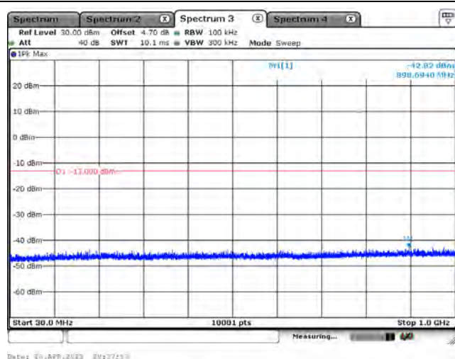
LTE Band 2_CH19100_20M_1RB0_QPSK_Below 1GHz
