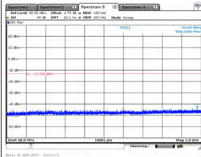
LTE Band 66_CH132322_1.4M_1RB0_QPSK_Below 1GHz
