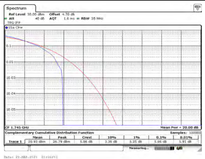
LTE Band 66_CH132322_5M_64-QAM_1RB0
