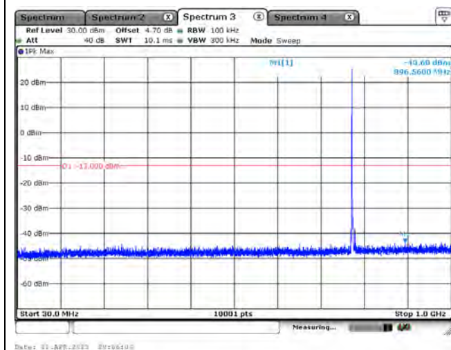
LTE Band 13_CH23230_5M_1RB0_QPSK_Below 1GHz
