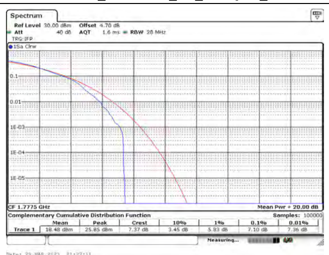
LTE Band 66_CH132647_5M_256-QAM_1RB24
