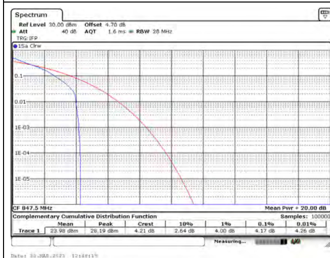
LTE Band 5_CH20635_3M_QPSK_1RB14
