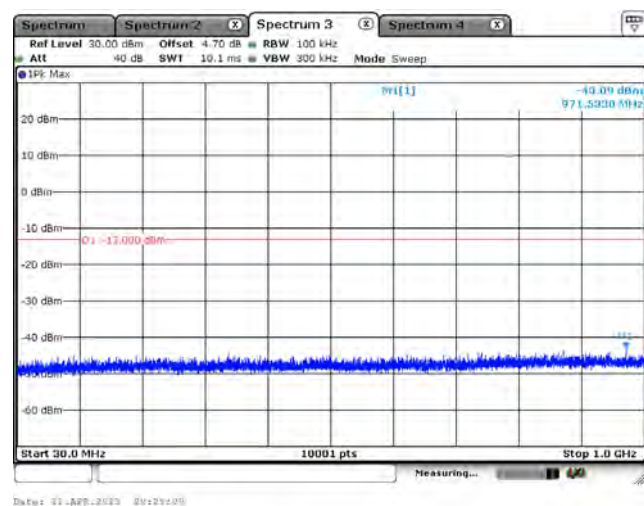
LTE Band 66_CH132322_10M_1RB0_QPSK_Below 1GHz
