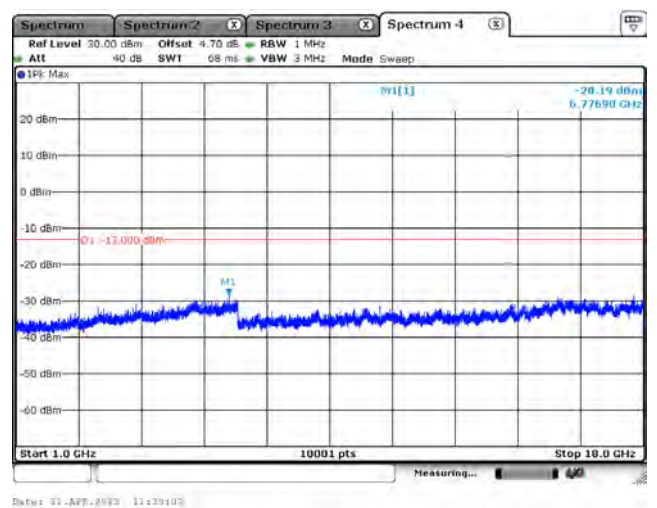
LTE Band 5_CH20525_1.4M_1RB0_QPSK_Above 1GHz
