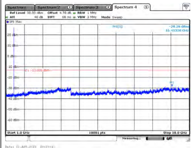
LTE Band 66_CH132322_10M_1RB0_QPSK_Above 1GHz
