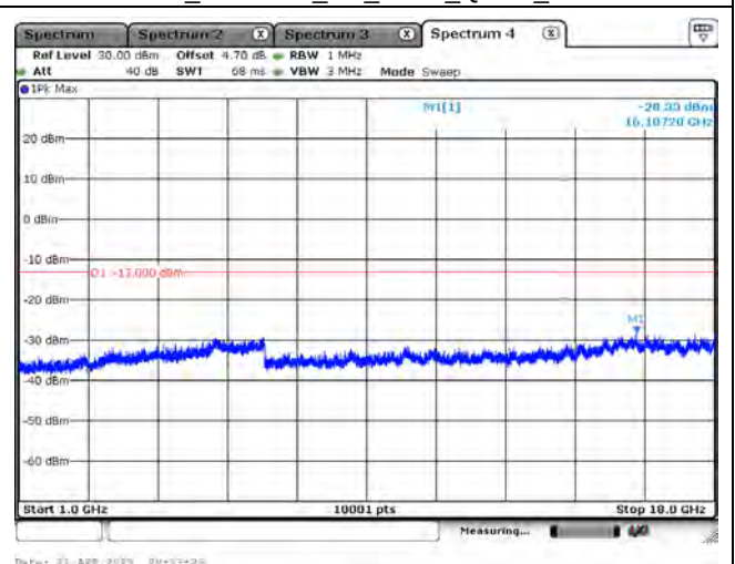
LTE Band 13_CH23255_5M_1RB0_QPSK_Above 1GHz
