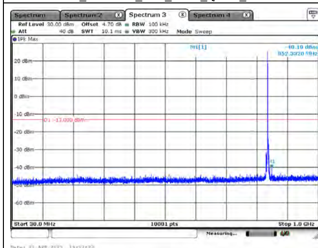
LTE Band 5_CH20600_10M_1RB0_QPSK_Below 1GHz
