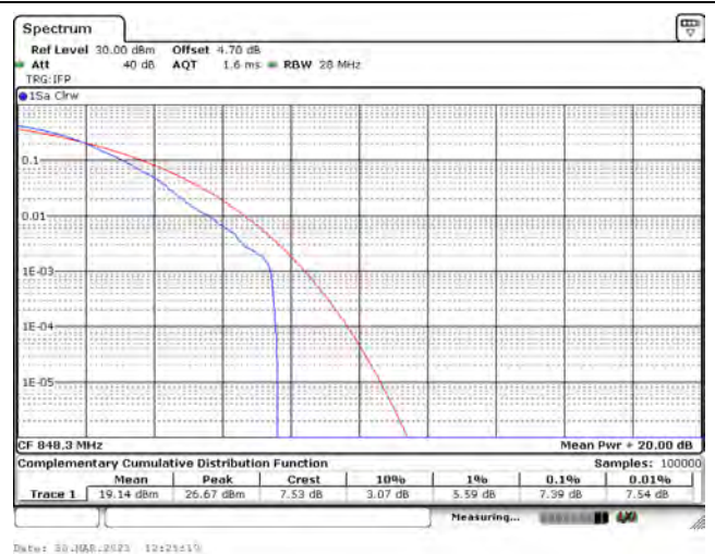
LTE Band 5_CH20643_1.4M_256-QAM_1RB5
