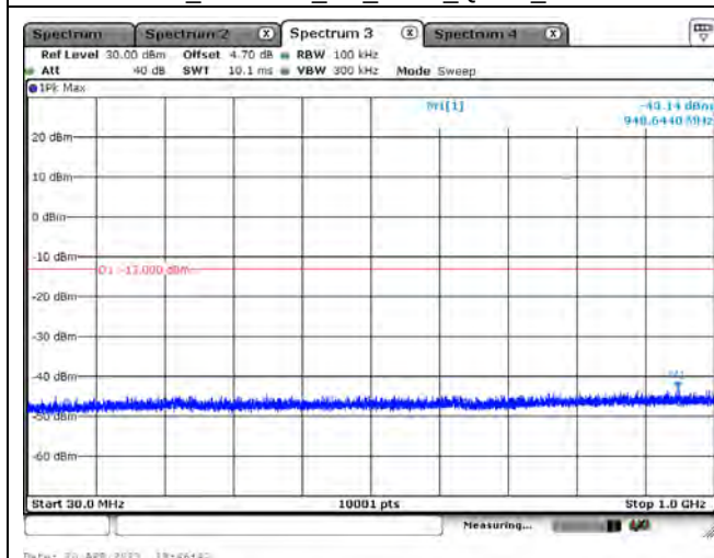
LTE Band 2_CH19185_3M_1RB0_QPSK_Below 1GHz
